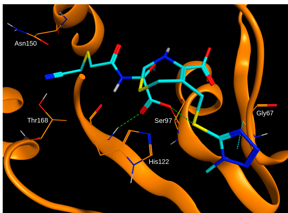
Figure 3. Binding mode of cefmetazole (carbon atoms in cyan) in ClpP obtained by molecular docking into Protein Data Bank (PDB) ID 2FZS using GOLD with the compound covalently attached to the hydroxyl oxygen of Ser97. Hydrogen bonds and C–H– \pi interactions are indicated as green and cyan dashed lines, respectively.
