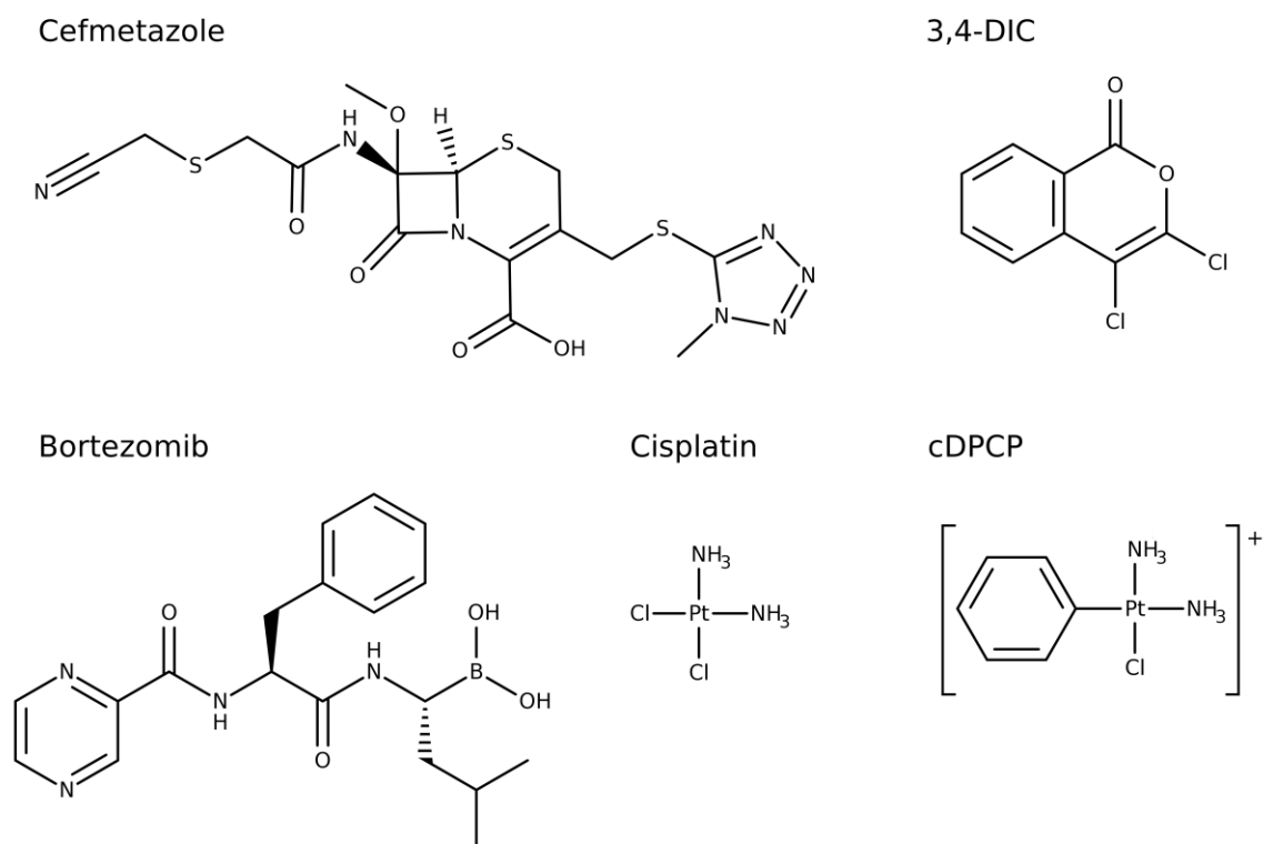
Figure 1. Structural formula of the five ClpP inhibitors identified in this study.
