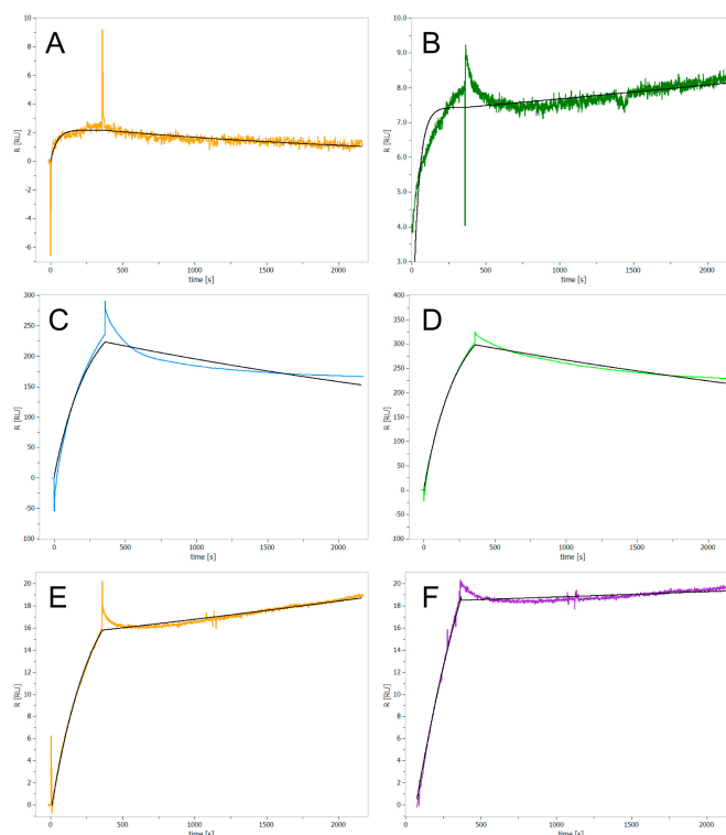
Figure 2. SPR sensorgrams of the ClpP inhibitors at 80 \mu M concentration. Each compound was injected over 7 min, followed by 30 min of dissociation time. (A) Bortezomib, (B) Cefmetazole, (C) cDPCP, (D) Cisplatin, (E) 3,4-DIC, and (F) Z-LY-CMK (covalent binder, control). The fitting curves of the SPR sensorgrams (black lines) were obtained using a 1:1 Langmuir interaction model.
