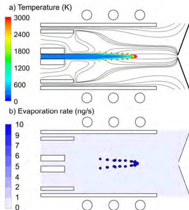
Figure 6. 2D trajectories of injected Cu particles, colored according to temperature, until they are evaporated, as well as the path lines of the injector gas, auxiliary gas and outer gas, colored in black (a), and 2D distribution of the Cu evaporation rate (b), for Cu particles with diameter of 1 \mu\text{m} and mass loading flow rate of 100 ng/s injected from the injector gas inlet. The other conditions are the same as in Figure 5.
