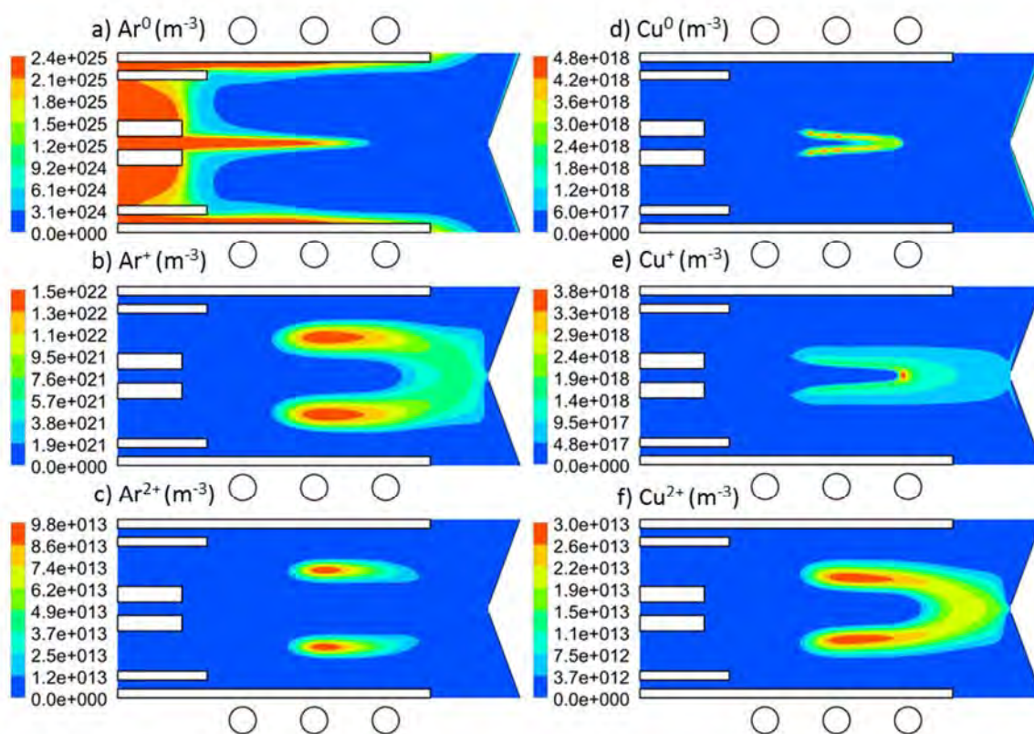
Figure 7. 2D number density profiles of the various species in the ICP: \text{Ar}^0 (a), \text{Ar}^+ (b), \text{Ar}^{2+} (c), \text{Cu}^0 (d), \text{Cu}^+ (e) and \text{Cu}^{2+} (f), for Cu particles with diameter of 1 \mu\text{m} and mass loading flow rate of 100 \text{ ng/s} injected from the injector gas inlet. The other conditions are the same as in Figure 5.
