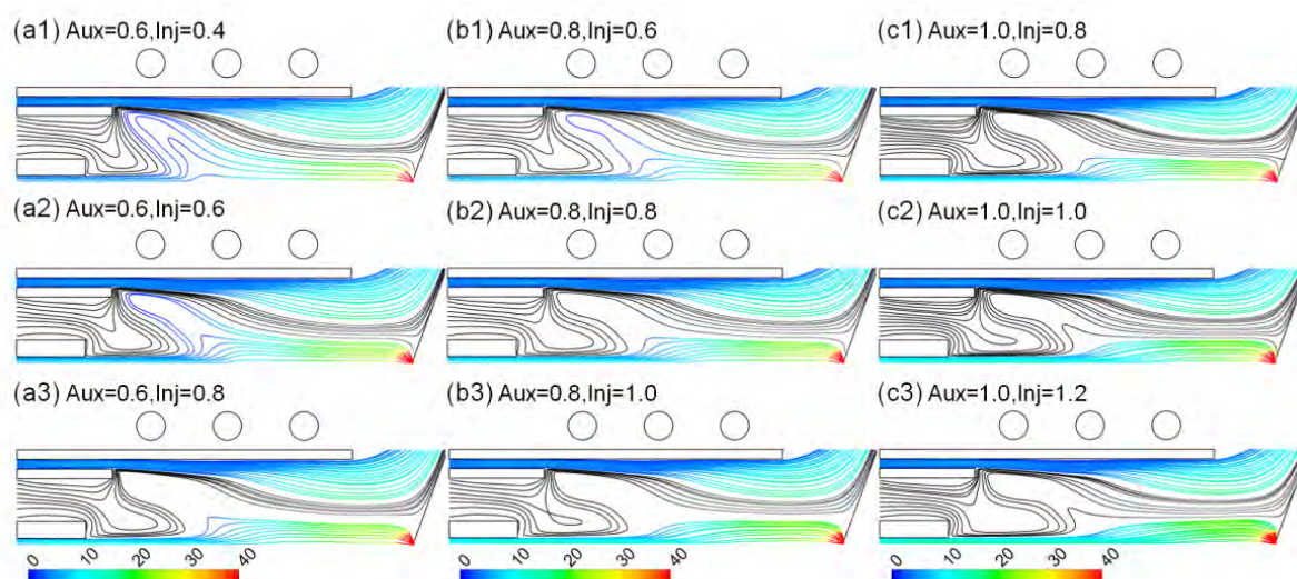
Figure 16. 2D gas flow velocity path lines originating from the injector gas and outer gas inlets, colored by velocity in m/s, and from the auxiliary gas inlet, colored in black, at (a) 0.6, (b) 0.8 and (c) 1.0 L/min of auxiliary gas flow rate. The injector gas flow rate is (1) lower than, (2) equal to and (3) higher than the auxiliary gas flow rate. Only half of the 2D axisymmetric torch is plotted. Reprinted from ref. 128 with permission from Elsevier.
