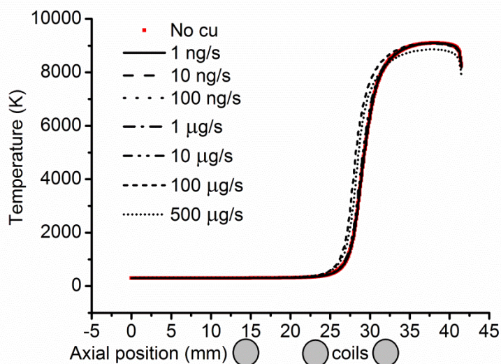
Figure 28. Plasma temperature along the central channel, for different Cu mass loading flow rates, as indicated in the legend. The other conditions are specified in Figure 5 and 6.
