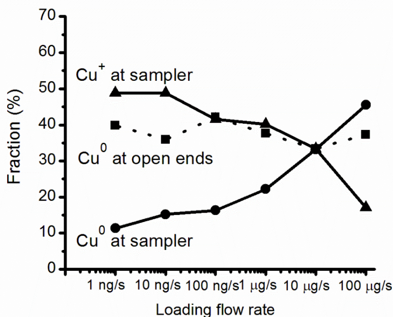
Figure 31. Fraction of \text{Cu}^+ and \text{Cu}^0 at the sampler and fraction of \text{Cu}^0 leaving at the open ends of the ICP, with respect to the total amount of Cu at the inlet, as a function of the Cu particle mass loading flow rate. The other conditions are specified in Figure 5 and 6.
