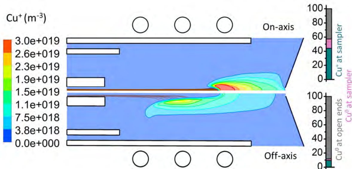
Figure 12. 2D \text{Cu}^+ ion number density profiles for on-axis (upper frame) and off-axis (bottom frame) injection, as well as trajectory of the Cu particles (brown path lines). At the right of the figure, the fraction of \text{Cu}^+ and \text{Cu}^0 at the sampler and fraction of \text{Cu}^0 leaving at the open ends of the ICP, with respect to the total amount of Cu at the inlet, for both on-axis and off-axis injection, are plotted. The other conditions are specified in Figure 5 and 6.
