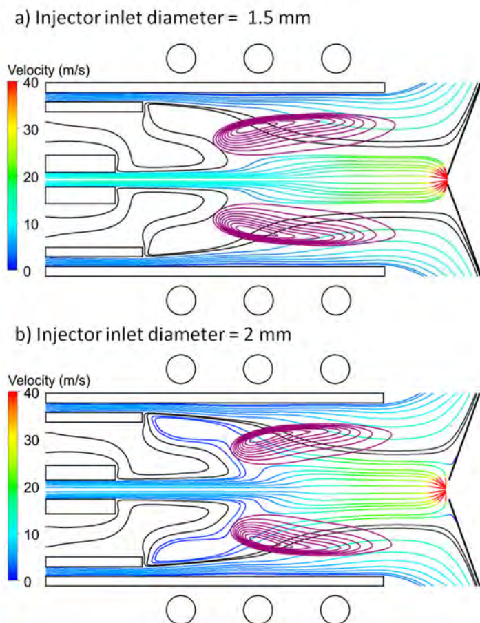
Figure 10. 2D gas flow velocity path lines for an injector inlet diameter of 1.5 mm (a) and 2.0 mm (b). The other conditions are the same as in Figure 5. Again, the color scale indicates the gas velocity for the injector gas and outer gas, while the auxiliary gas flow path lines are colored in black, and the purple contours indicate the region of maximum power coupling. Reproduced from ref. 130 with permission from the Royal Society of Chemistry.
