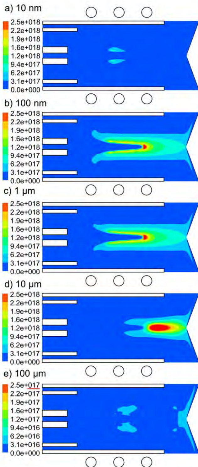
Figure 26. 2D \text{Cu}^+ ion number density profiles for different Cu particle diameters. The other conditions are specified in Figure 5 and 6. Note that the color scale for panel (e) indicates 10x lower values, as otherwise no density profile would be visible here.
