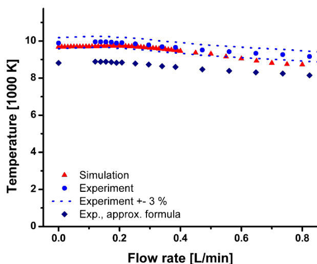
Figure 3. Calculated and measured plasma temperatures as a function of injector gas flow rate. Reprinted with permission from ref. 126 Copyright 2011 American Chemical Society.
