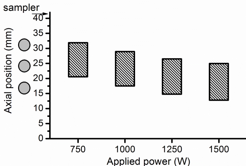
Figure 23. Spatial range of evaporation in the axial direction, as a function of applied power. The other conditions are specified in Figure 5 and Figure 6.
