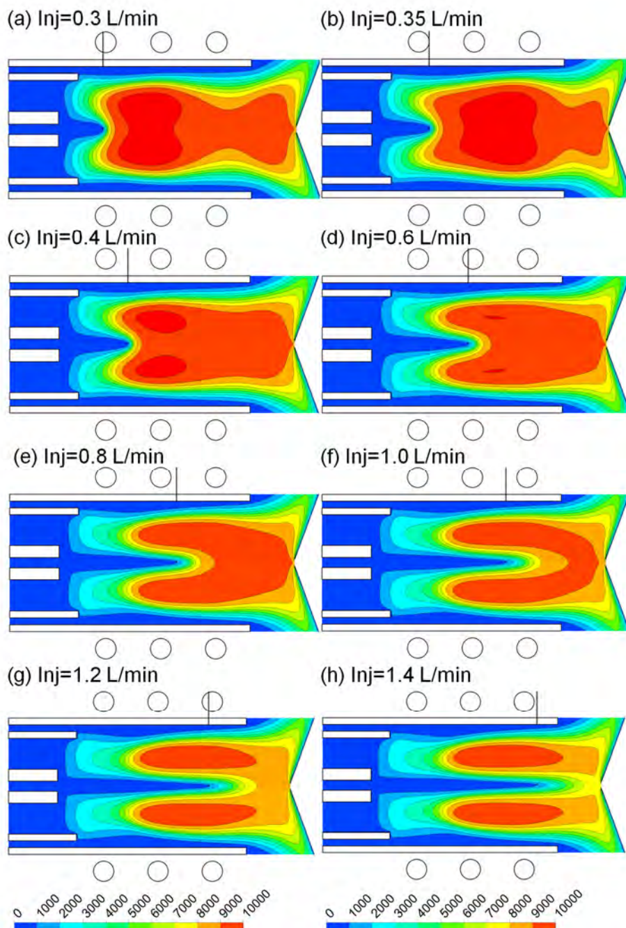
Figure 13. 2D plasma temperature profiles (K), at different values of the injector gas flow rate, ranging from 0.3 to 1.4 L/min. The other conditions are the same as in Figure 5. The small black lines above each plot indicate the length of the cool central channel. Reprinted from ref. 128 with permission from Elsevier.
