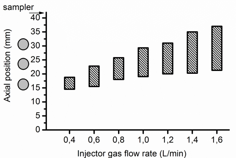
Figure 17. Spatial range of evaporation in the axial direction, as a function of injector gas flow rate. The other conditions are specified in Figure 5 and Figure 6.
