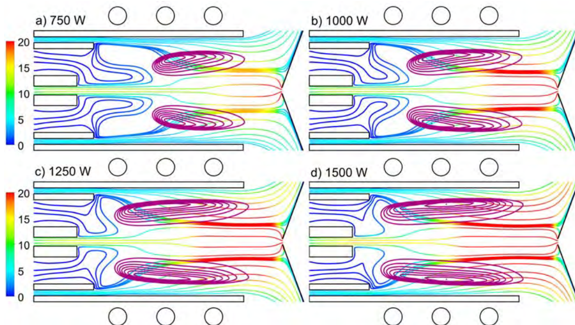
Figure 22. 2D gas flow velocity path lines of the injector gas, auxiliary gas and outer gas, colored by velocity in m/s, at an applied power of 750 W (a), 1000 W (b), 1250 W (c) and 1500 W (d). The other conditions are the same as in Figure 5. The purple contours indicate the region of maximum power coupling.
