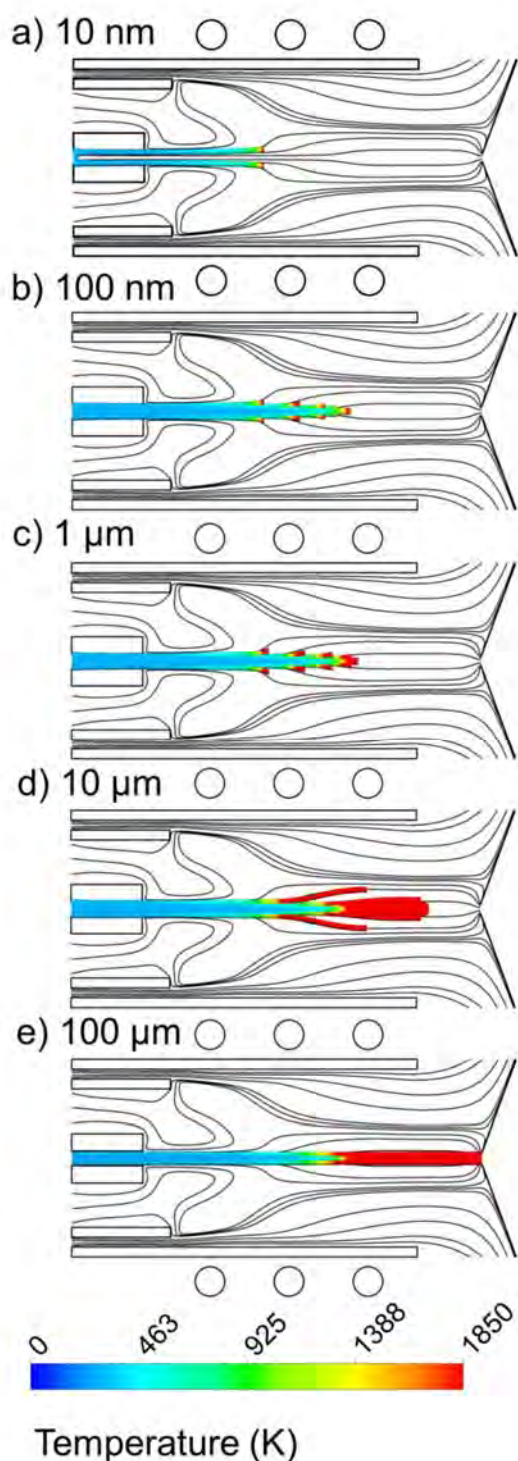
Figure 25. Effect of particle diameter on the 2D trajectories of Cu particles, colored according to their temperature, as well as the Ar gas flow path lines originating from injector gas, auxiliary gas and outer gas, colored in black. The other conditions are specified in Figure 5 and 6.
