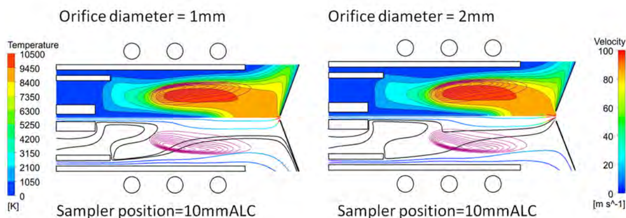
Figure 9. 2D plasma temperature profiles (upper frames) and gas velocity path lines (lower frames) for a sampler orifice diameter of 1 mm (left panel) and 2 mm (right panel). The other conditions are the same as in Figure 5. The color scale indicates the gas velocity for the injector gas and outer gas, while the auxiliary gas flow path lines are colored in black, and the purple contours indicate the region of maximum power coupling. Reproduced from ref. 129 with permission from the Royal Society of Chemistry.
