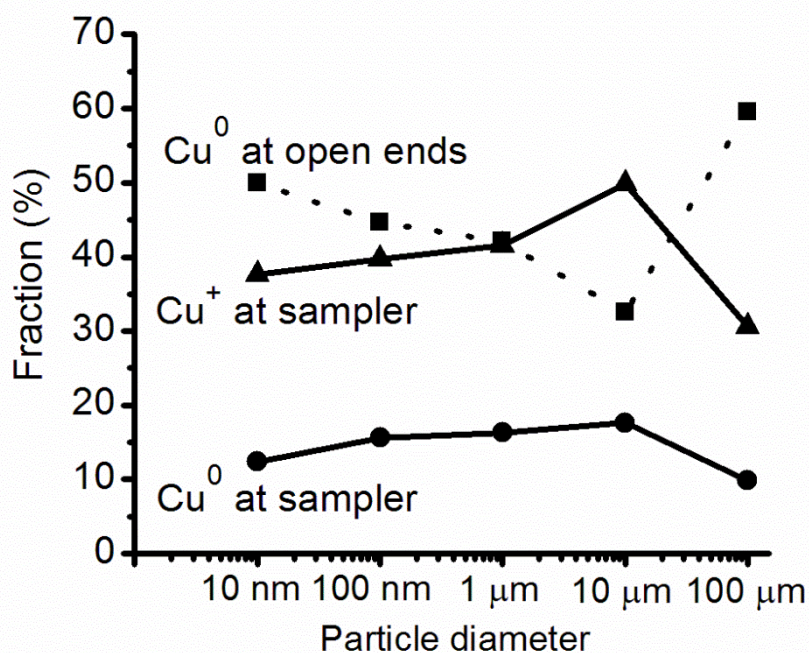
Figure 27. Fraction of \text{Cu}^+ and \text{Cu}^0 at the sampler and fraction of \text{Cu}^0 leaving at the open ends of the ICP, with respect to the total amount of Cu at the inlet, as a function of the particle diameter. The other conditions are specified in Figure 5 and 6.
