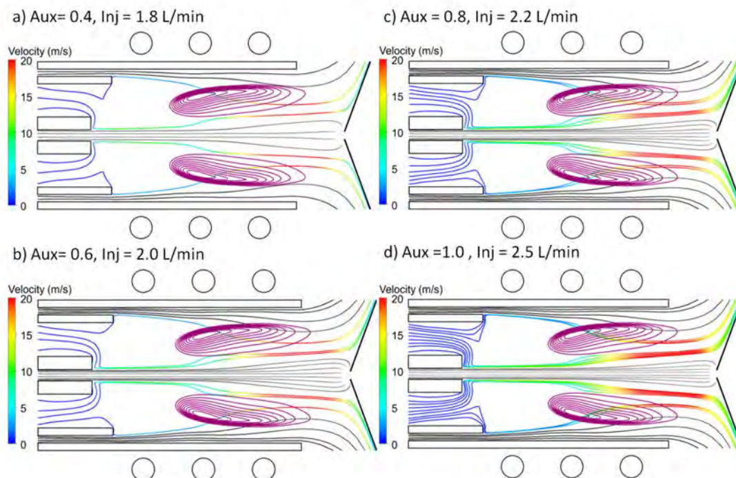
Figure 15. 2D gas flow velocity path lines originating from the auxiliary gas inlet, colored by velocity in m/s, as well as from the injector gas and outer gas inlets, colored in black, at different values of the injector gas and auxiliary gas flow rates, as indicated above the panels. For each auxiliary gas flow rate given (Aux), the corresponding injector gas flow rate (Inj) indicates the transition point, or minimum value needed to avoid (major) recirculation in the auxiliary gas. The other conditions are the same as in Figure 5. The purple contours indicate the region of maximum power coupling.
