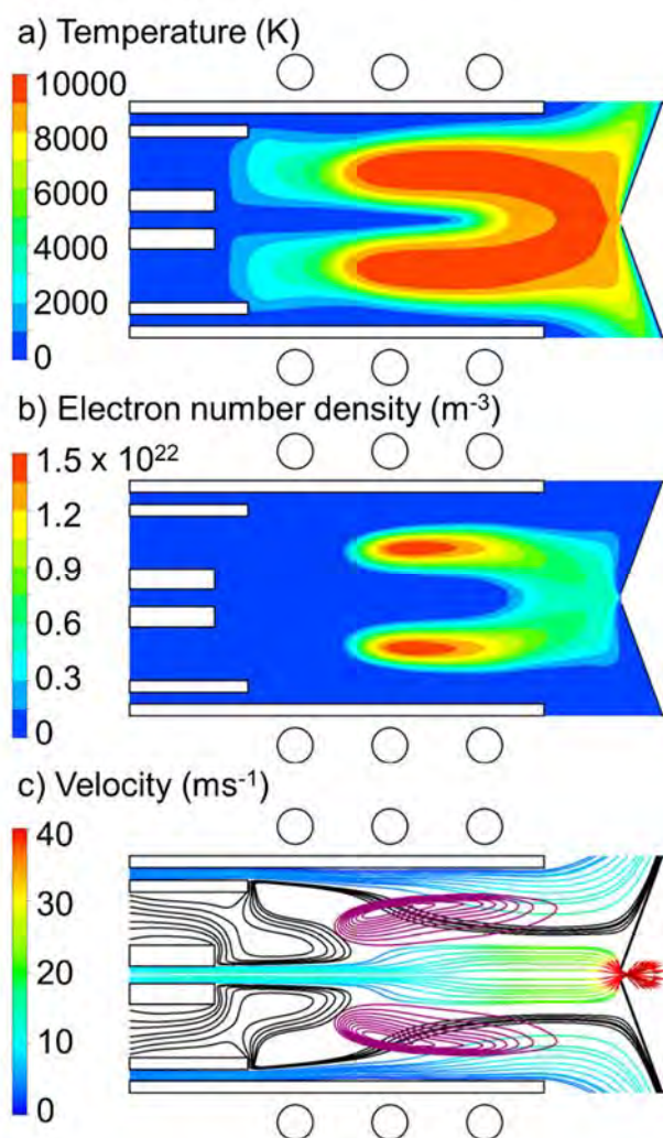
Figure 5. 2D profiles of the plasma temperature (a), electron density (b) and the gas flow velocity path lines (c), calculated for 1 L/min injector gas, 0.4 L/min auxiliary gas, and 12 L/min outer gas flow rate, and a plasma power of 1000 W. The diameters of the injector inlet and sampler orifice are 1.5 and 1 mm, respectively. The sampling cone is placed 10 mm from the load coil. Note that the color scale in panel (c) indicates the gas velocity for the injector gas and outer gas, while the auxiliary gas flow path lines are colored in black, to distinguish them from the injector gas and outer gas. The purple contours in panel (c) indicate the region of maximum power coupling.
