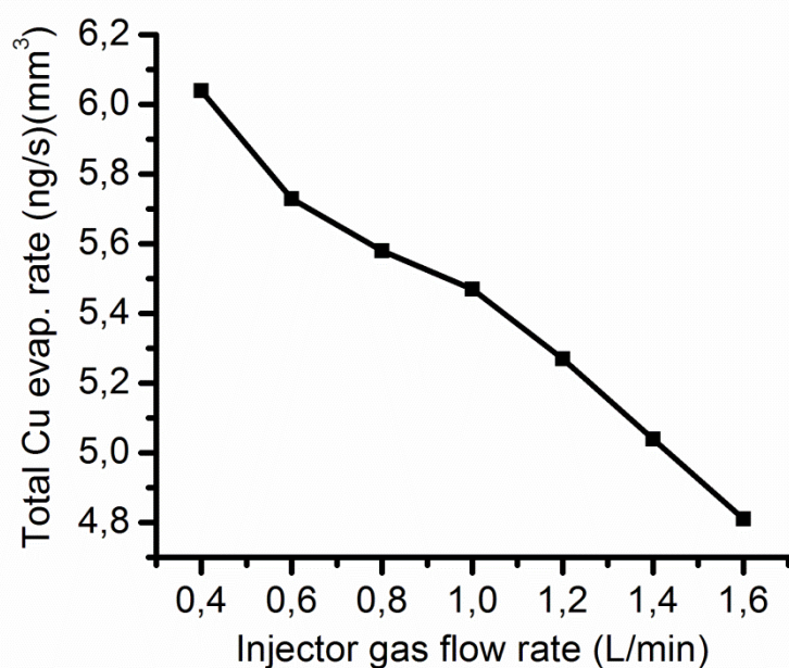
Figure 18. Total Cu sample evaporation rate, integrated over the entire torch, as a function of the injector gas flow rate. The other conditions are specified in Figure 5 and 6.
