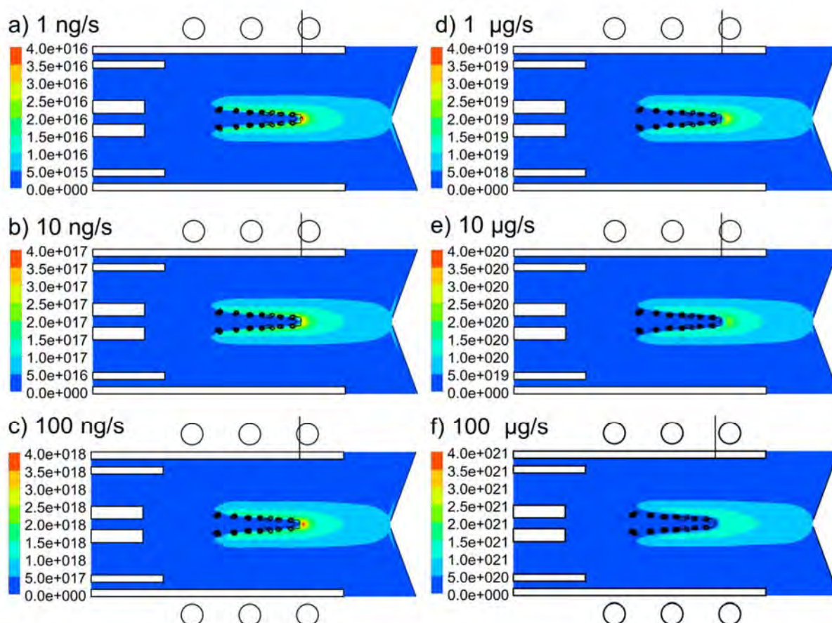
Figure 30. 2D \text{Cu}^+ ion number density profiles, as well as the contours of the Cu evaporation rate, for 6 different Cu particle mass loading flow rates. The other conditions are specified in Figure 5 and 6. The maximum position of evaporation is indicated with the thin black line above each panel.
