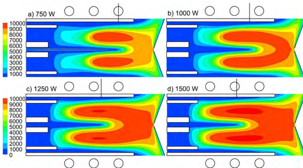
Figure 21. 2D plasma temperature profiles, at an applied power of 750 W (a), 1000 W (b), 1250 W (c) and 1500 W (d). The other conditions are the same as in Figure 5. The small black lines above each panel indicate the length of the cool central channel.
