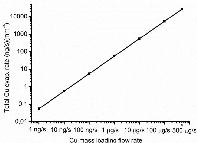
Figure 29. Total Cu sample evaporation rate, integrated over the entire torch, as a function of the Cu particle mass loading flow rate. The other conditions are specified in Figure 5 and 6.
