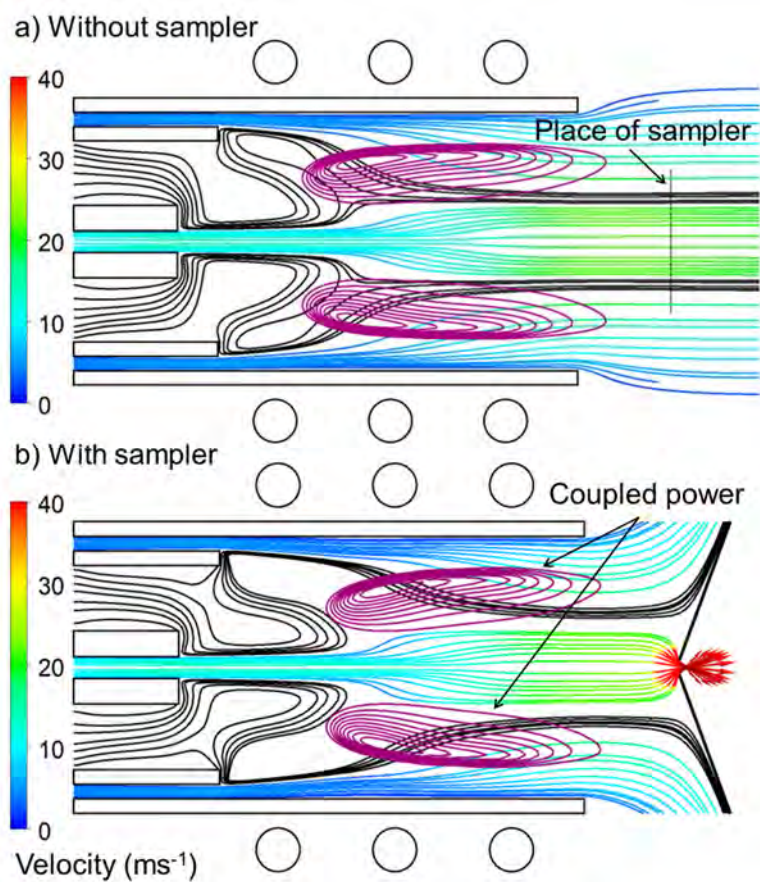
Figure 8. 2D gas flow velocity path lines, without (a) and with (b) sampling cone, for the same conditions as in Figure 5. Again, the color scale indicates the gas velocity for the injector gas and outer gas (in m/s), while the auxiliary gas flow path lines are colored in black, and the purple contours indicate the region of maximum power coupling.
