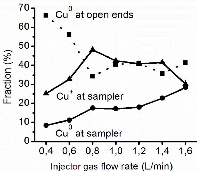
Figure 20. Fraction of \text{Cu}^+ and \text{Cu}^0 at the sampler and fraction of \text{Cu}^0 leaving at the open ends, with respect to the total amount of Cu at the inlet, as a function of the injector gas flow rate. The other conditions are specified in Figure 5 and 6.
