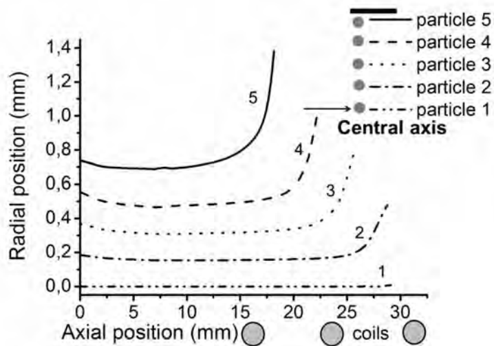
Figure 11. Radial position of 5 different Cu particles (with different injection positions; see legend) as a function of their axial position in the ICP, to illustrate the effect of their injection position on their trajectory. The conditions are the same as in Figure 5 and 6. The positions of the load coils are also indicated in the figure, for clarity.
