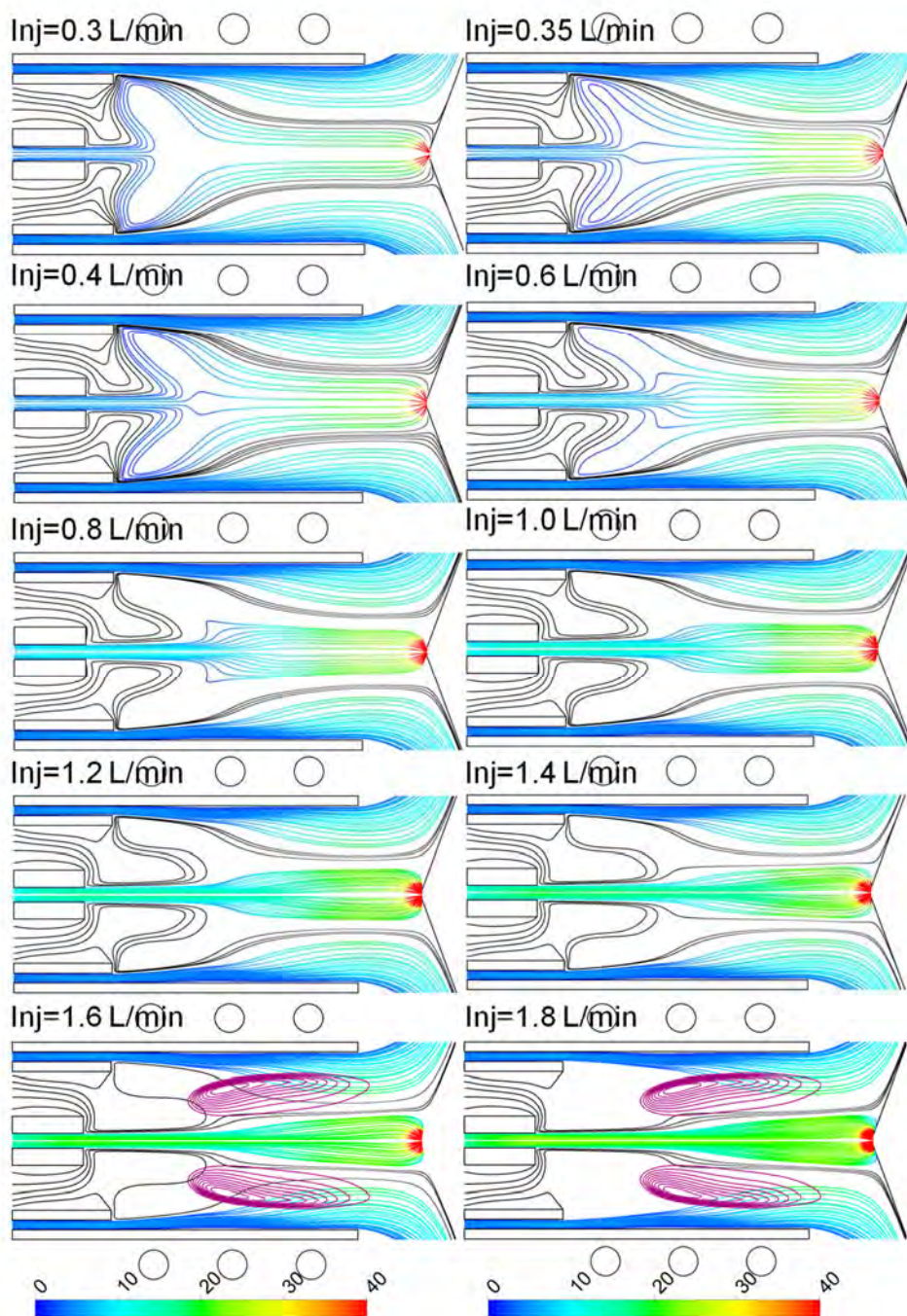
Figure 14. 2D gas flow velocity path lines originating from the injector gas and outer gas inlets, colored by velocity in m/s, and from the auxiliary inlet, colored in black, at different values of the injector gas flow rate, ranging from 0.3 to 1.8 L/min. The other conditions are the same as in Figure 5. The purple contours in the two bottom frames indicate the region of maximum power coupling. Reprinted from ref. 128 with permission from Elsevier.
