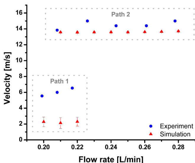
Figure 4. Calculated and measured velocities as a function of injector gas flow rate, for two different regions inside the ICP, i.e., path 1 corresponds to the region between the first and second winding of the coil, whereas path 2 corresponds to the region between the second and third winding of the coil. Reprinted with permission from ref. 126 Copyright 2011 American Chemical Society.
