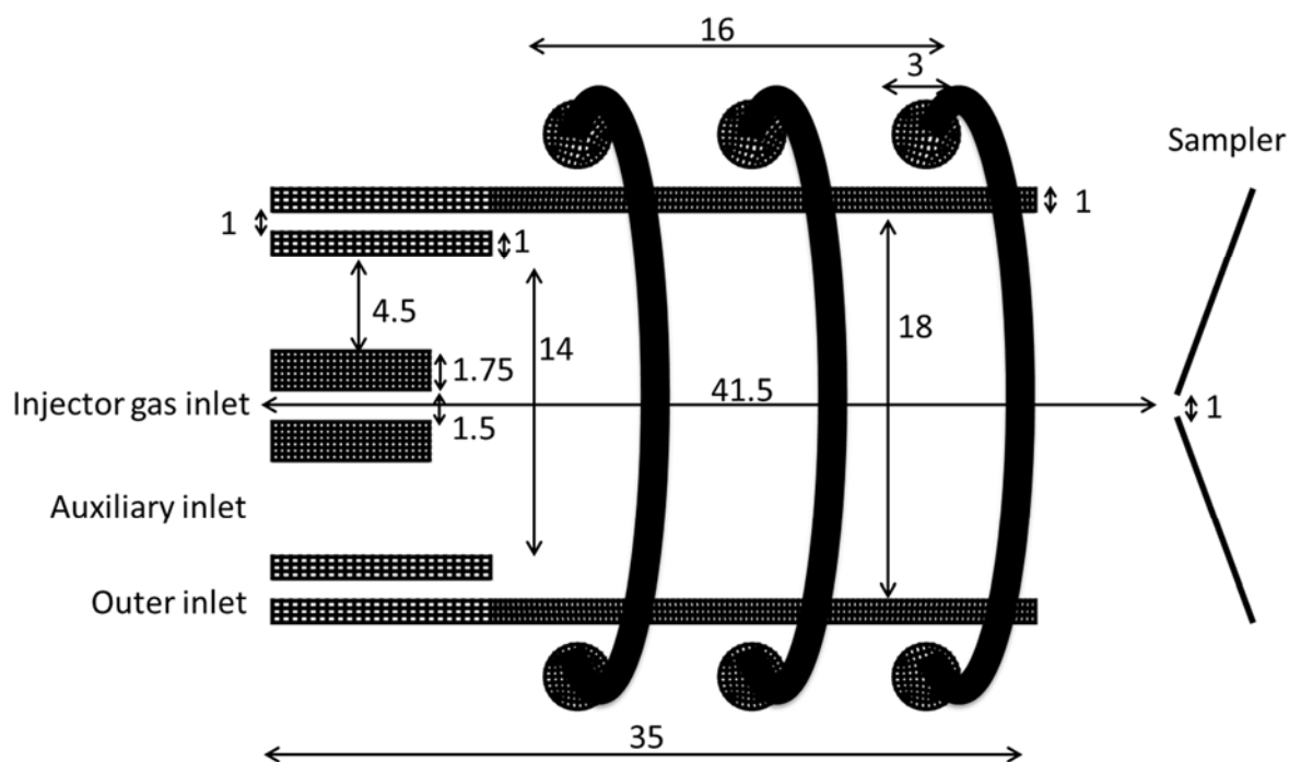
Figure 1. Schematic picture of the ICP geometry assumed in the 2D axisymmetric model. The dimensions are given in mm. Note that the distance between sampler and load coil, as well as the diameter of the sampler and injector gas inlet were varied in our simulations (see the range in Table 1).
