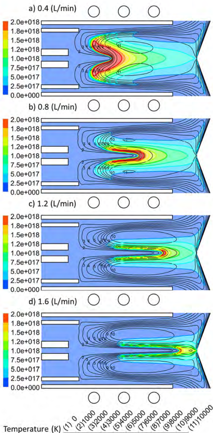
Figure 19. 2D \text{Cu}^+ ion number density profiles at four different injector gas flow rates, i.e., 0.4 (a), 0.8 (b), 1.2 (c) and 1.6 (d) L/min, as well as the plasma temperature profiles (black contours) ranging from 0 to 10,000 K (see explanation of the labels at the bottom of the figure). The other conditions are specified in Figure 5 and 6.
