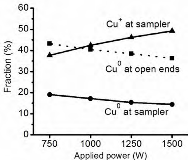
Figure 24. Fraction of \text{Cu}^+ and \text{Cu}^0 at the sampler and fraction of \text{Cu}^0 leaving at the open ends of the ICP, with respect to the total amount of Cu at the inlet, as a function of the applied power. The other conditions are specified in Figure 5 and 6.
