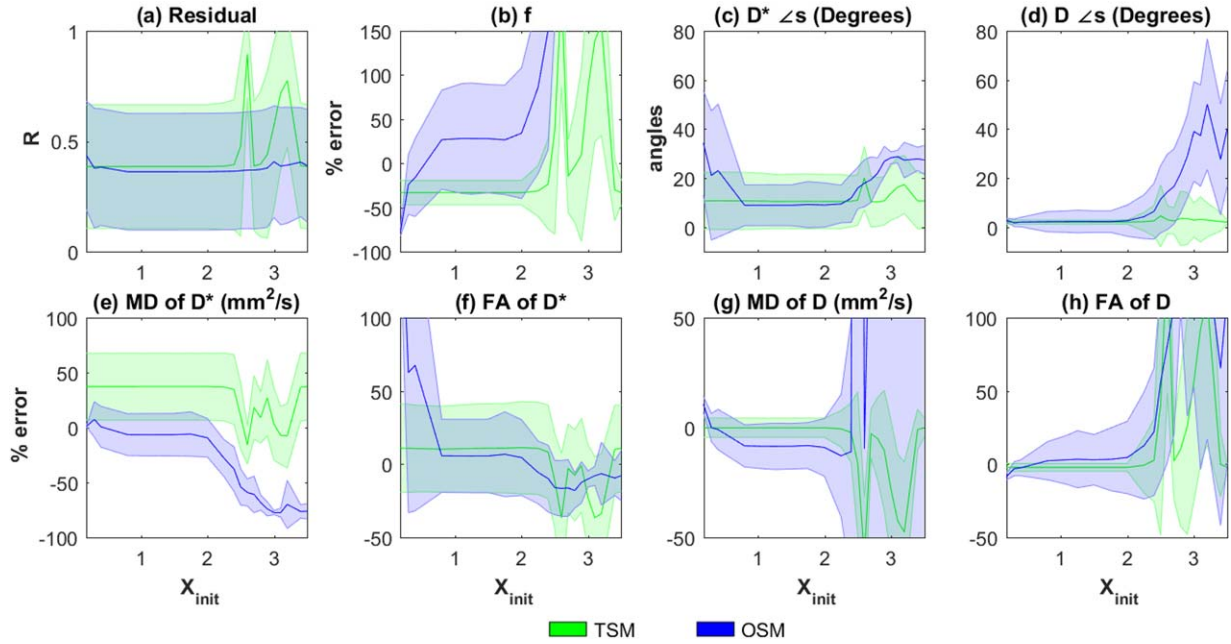
FIG. 2. Dependence on initialization on TSM and OSM estimates. Plots of (a) R , (b) percentage errors in f , (c) error in angles (in degrees) of estimated D^* and (d) D , percentage errors in (e) MD of D^* , MD( D^* ), (f) FA of D^* , FA( D^* ), (g) MD of D , MD( D ), (h) FA of D , FA( D ) plotted against X_{init} , Equation [11]. In all the plots, the thick lines represent the mean of the estimated values from the 500 noisy samples of Y and the shaded region represents the standard deviation. Here X_{init} varies from 0.2 to 3.5.
