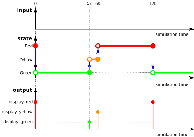
Figure 3: Stepping through a state trace.
