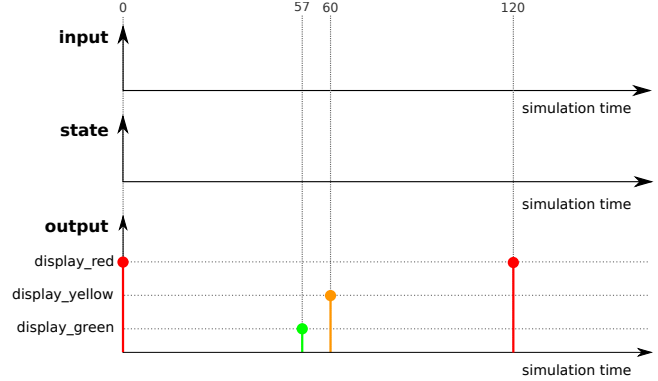
Figure 2: Stepping through an input/output trace.
