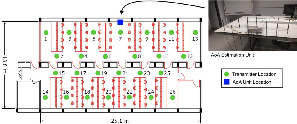
Fig. 1. The experimental setup. It constitutes two parallel computer classrooms of dimensions 25.1m×6.9m each. 780 DASH7 signals were transmitted from 26 different locations in both rooms (30 signals per location).
