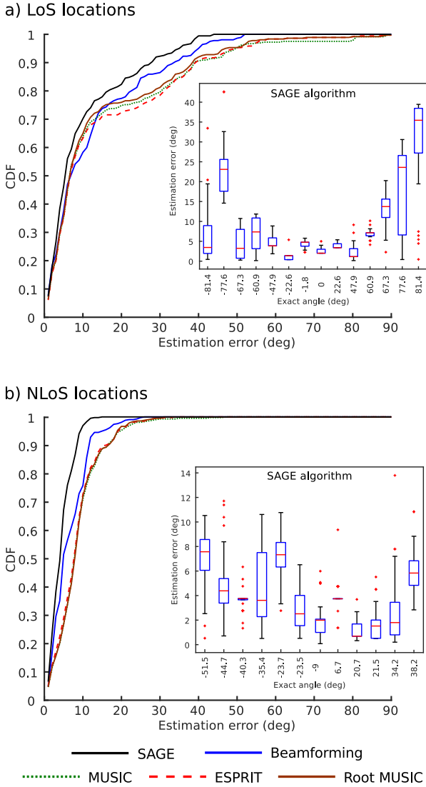
Fig. 2. The CDF and the boxplot (inner figures) for the AoA estimation error of all the received signals from the LoS and the NLoS locations, respectively. The CDF figures show the AoA estimation error as estimated from all the deployed AoA estimation algorithms. The boxplot figures, on the other hand, provide the AoA estimation error from the SAGE algorithm only. Every boxplot represents the estimation error from a specific location (i.e. 26 boxplot graphs in total).
