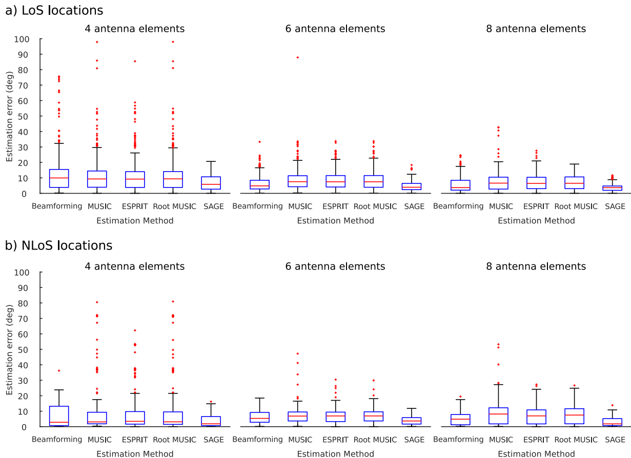
Fig. 3. The boxplot graphs of the AoA estimation error from the various AoA estimation algorithms for different deployed array antenna aperture. Both the LoS and the NLoS locations were considered.
