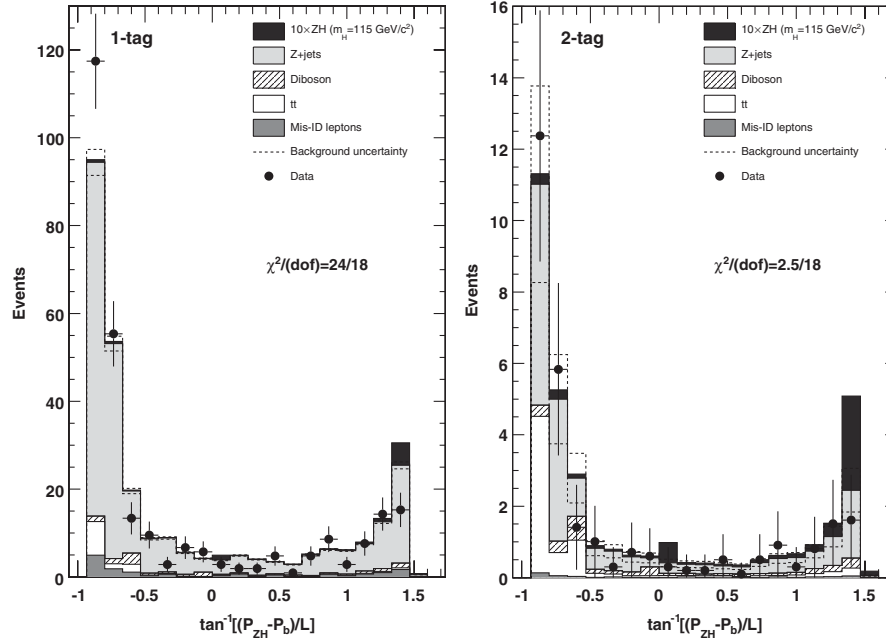
FIG. 1. The distribution of \tan^{-1}D where the discriminant D = (P_{ZH} - P_b)/L for expected backgrounds and data for events with one (left) and two (right) b tags. The expected signal ( \times 10 ) is overlaid. The \chi^2 is based on the data and total background expectation as shown, using the expected statistical uncertainties and the bin-to-bin uncorrelated systematic uncertainties on the background.
