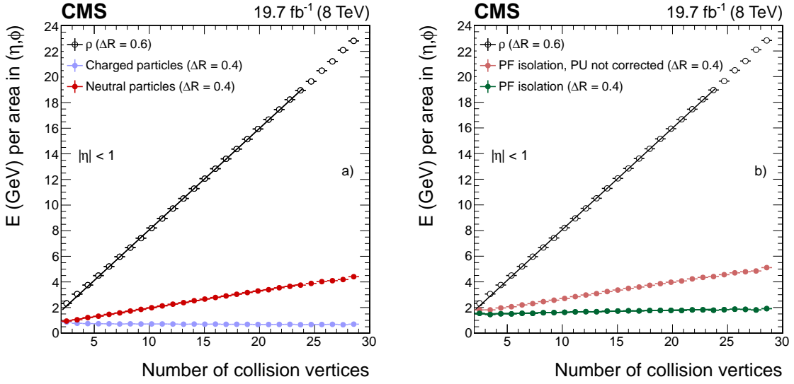
Figure 20. Average energy density as a function of the number of reconstructed proton-proton collision vertices, for electron candidates with p_T > 20\text{GeV} and |\eta| < 1 from data dominated by Z \rightarrow e^+e^- events. The energy density \rho (open dots) is shown, along with each component of the particle isolation: a) neutral particles (red dots) and charged particles associated with the vertex (blue dots), and b) before (pink dots) and after (green dots) the correction for pileup on PF isolation.
