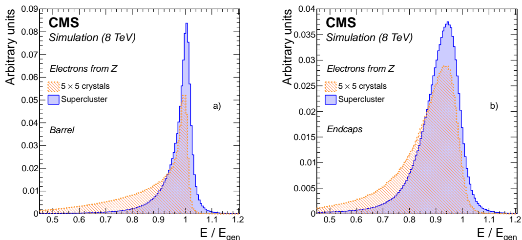
Figure 3. Comparison of the distributions of the ratio of reconstructed over generated energy for simulated electrons from Z boson decays in a) the barrel, and b) the endcaps, for energies reconstructed using superclustering (solid histogram) and a matrix of 5 \times 5 crystals (dashed histogram). No energy correction is applied to any of the distributions.
