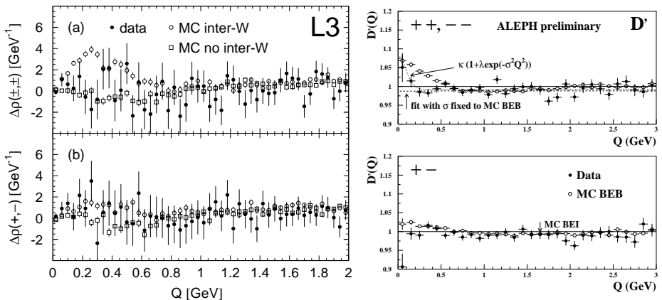
Fig. 1. Left: The \Delta\rho(Q) distribution, measured by the L3 collaboration. Right: The D'(Q) distribution measured by ALEPH. In both figures, the LUBOEI BE32 models, tuned to hadronic Z^0 data for each individual experiment, including either only BEC inside one W or BEC between all identical bosons are superimposed.
