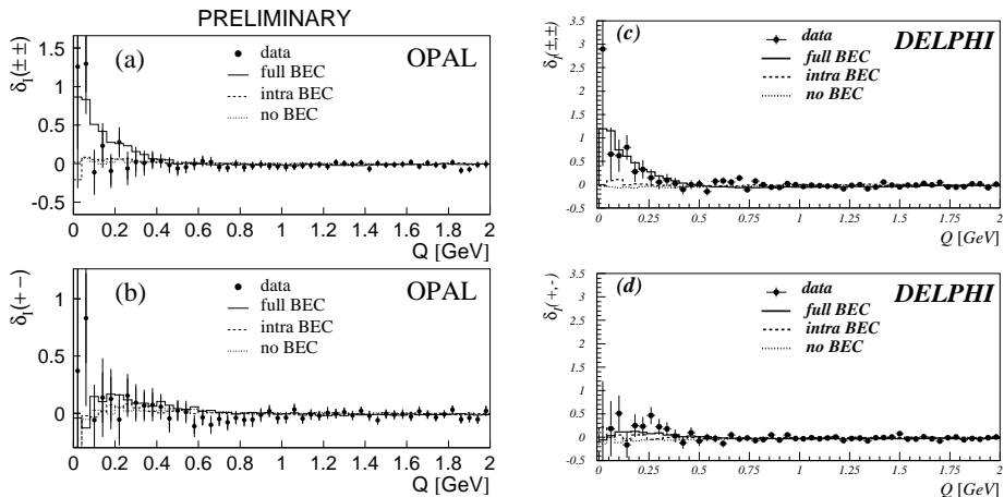
Fig.2. The genuine inter- W correlation function, \delta_I(Q) , for like sign (top) and unlike-sign (bottom) particle pairs analyzed by OPAL (left) and DELPHI (right). Several BEC scenarios implemented with BE32 are superimposed.
