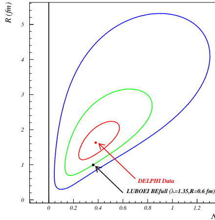
Fig. 4. The one, two and three sigma contours of the measured correlation strength \Lambda and R parameter, taken from a fit by DELPHI to D(Q) with expression 10.
