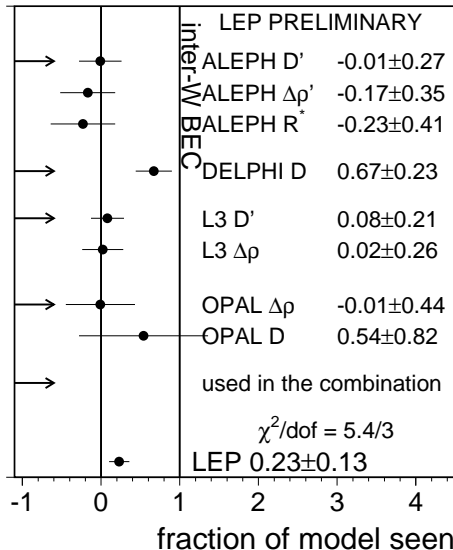
Fig. 3. The fraction of the full BE32 model seen by each experiment, using different techniques. The results with arrows are considered for combination.
