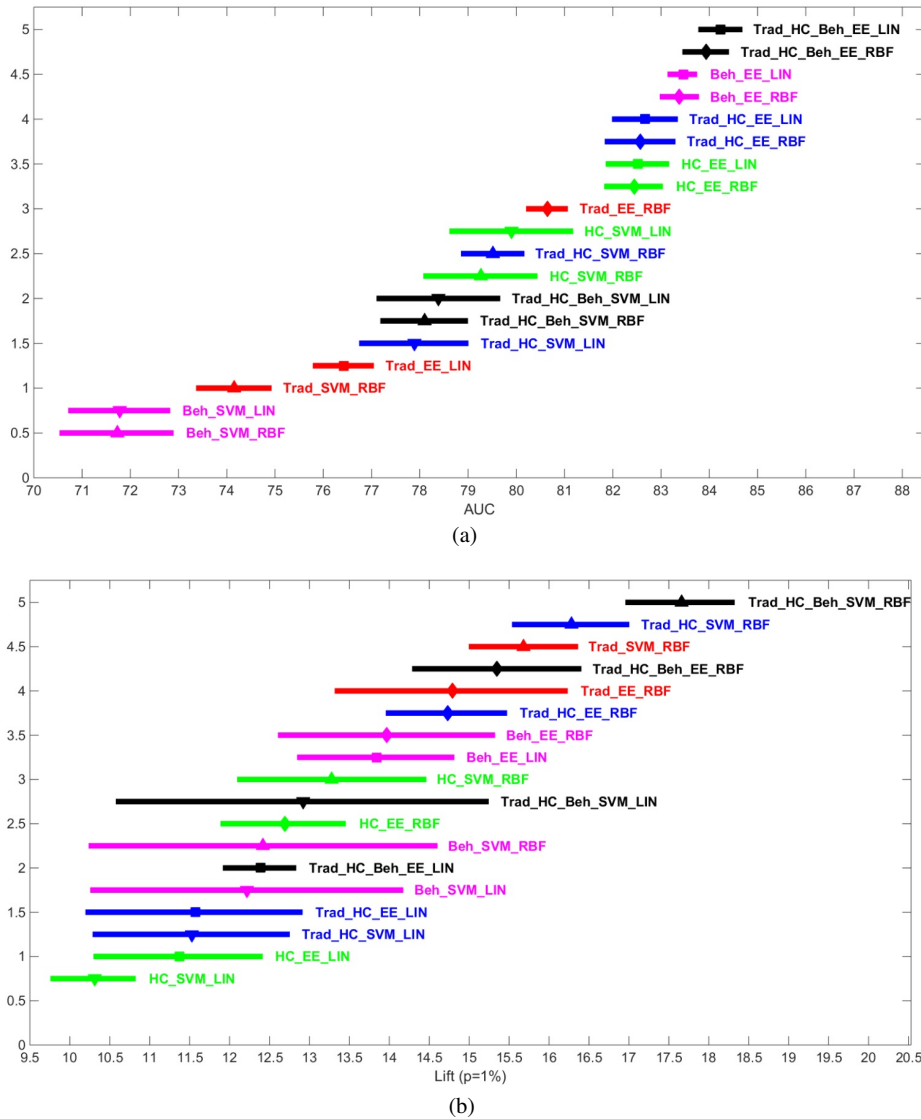
Fig. 5 Combining the data sources into data ensemble models. Additionally, the best performances of the individual data sources are repeated for convenience. Results showing the (a) AUC and (b) lift ( p = 1\% ) performance across ten folds of test data
