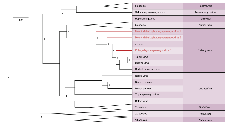
Fig. 2 Maximum clade credibility tree of 69 currently known paramyxovirus species. The phylogeny imputed from the concatenated sequence of the N, P, M, F, G and L proteins of 69 known paramyxovirus species shows that MMLPV-1, MMLPV-2 and PMPV-1 (marked in red) cluster with perfect support as separate species together with JPV, BeiPV, TImPV and rodent PV. Branches of recognized genera that contain multiple species have been collapsed. An expanded version of this tree is given in Additional file 1: Figure S1. A version of this tree based only on the L protein but including the recently discovered fish paramyxoviruses is given in Additional file 2: Figure S2. Branch lengths are scaled and represent the number of amino acid substitutions per site. Numbers at the different nodes indicate the posterior support for a cluster. GenBank accession numbers of all used sequences are provided in Additional file 3: Table S1
