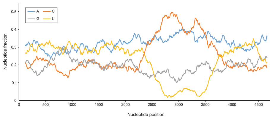
Fig. 1 Nucleotide composition of the PMPV-1 G gene. A sliding window view of the nucleotide composition of the PMPV-1 G gene, using 5% of the gene length as window size, shows that this gene has a low GC-content, comparable to the rest of the PMPV-1 genome, as well as a ~ 1400 nt-long region that is marked by a near-absolute absence of uracils (< 5%) and an abundance of cytosines (up to 50%). The unique nucleotide composition of the PMPV-1 G gene is also reflected in the amino acid composition of the corresponding G protein (see Fig. 5)
