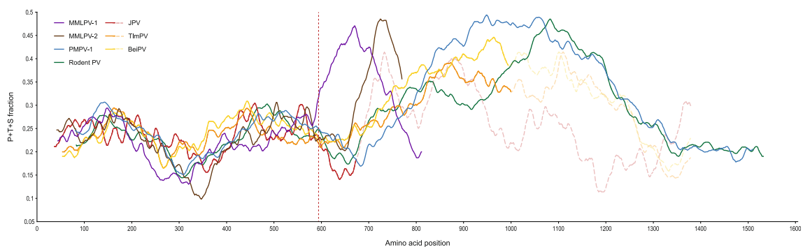
Fig. 5 Sliding window overview of the amino acid composition of all Jeilongvirus G proteins. The used window size for each protein is 10% of the respective protein length. The dotted red line represents the average length of paramyxovirus G proteins. All Jeilongvirus G proteins are marked by the presence of an otherwise absent C-terminal region, marked by a high, yet variable abundance of P/T/S (up to 50%). In the genomes of JPV, BeiPV and TImPV, the G gene is divided into two ORFs, G and X. A single mutation/insertion, however, suffices to join these two ORFs into a single ORF covering the entire G gene. The P/T/S fraction of the resulting hypothetical BeiPV and TImPV G proteins (yellow/orange dashed lines) is similar to those of the Rodent PV and PMPV-1 G proteins. For JPV, which is more closely related to MMLPV-1/2 (Fig. 2, Additional file 1: Figure S1), this effect is less pronounced, although a narrow peak in P/T/S-abundance, similar to the MMLPV-2 peak, can be observed in the resulting hypothetical JPV G protein (dashed red line)
