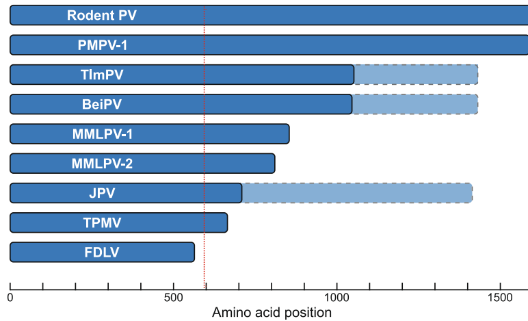
Fig. 4 Comparison of the G ORFs of all ‘Jeilongviruses’. The G ORFs of the seven known ‘Jeilongviruses’ show a remarkable variation in size, and all of them are larger than those of other paramyxoviruses. The dashed red line marks the average size of a paramyxovirus G ORF. The G ORFs of Tupaia paramyxovirus (TPMV) and Fer-de-lance virus (FDLV) are included to illustrate both the exceptional size of the ‘Jeilongvirus’ G ORFs and their mutual variation, as these two viruses have the largest and smallest G ORFs of all non-‘Jeilongvirus’ paramyxoviruses, respectively. The light blue extensions indicate the complete size of the BeiPV, TImPV and JPV G genes, including the X ORFs
