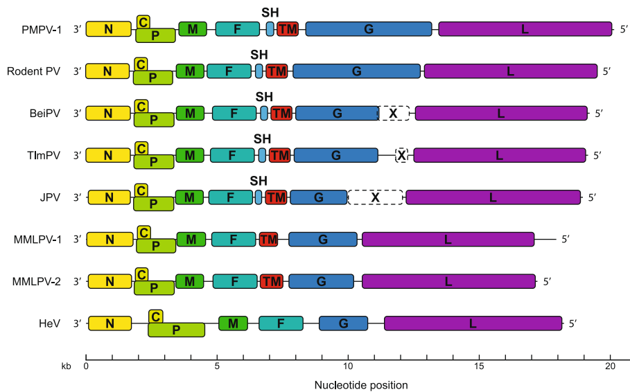
Fig. 3 Genome organization of all known ‘Jeilongviruses’. All ORFs are drawn to scale. The X ORF (dashed lines) is found only in the genomes of BeiPV, TImPV and JPV, and is considered part of the G gene. The SH gene is found only in a limited number of paramyxoviruses, while the TM gene appears to be a unique feature of members of the putative genus ‘Jeilongvirus’. Hendra virus (HeV) is included as a reference non-‘Jeilongvirus’ genome
