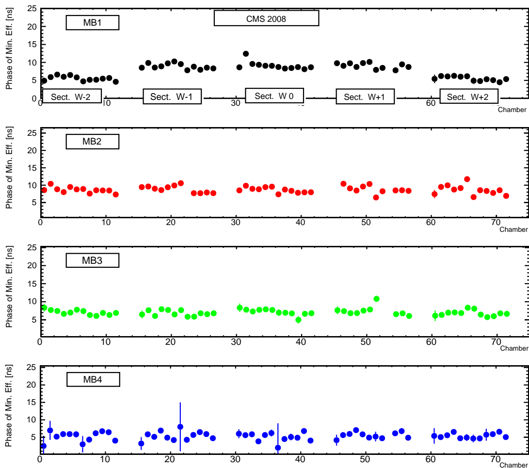
Figure 9. Phase of the minimum of HH quality DTLT efficiency. On the x axis, each entry corresponds to one chamber ordered by sector (1 to 12), and by wheel (-2 to +2). Some chambers are missing for which the triggers primitives were not read out, or a high voltage channel was disconnected.
