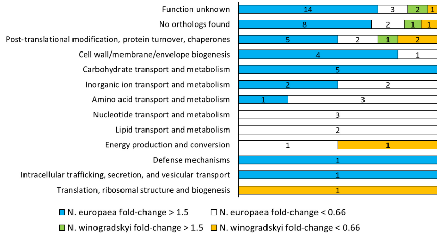
FIGURE 2 | Clusters of Orthologous Groups (COGs) classification of N. europaea and N. winogradskyi proteins with a significant fold change (higher than 1.5 or lower than 0.66; p < 0.05 ) after exposure to 30 mS \text{cm}^{-1} .
