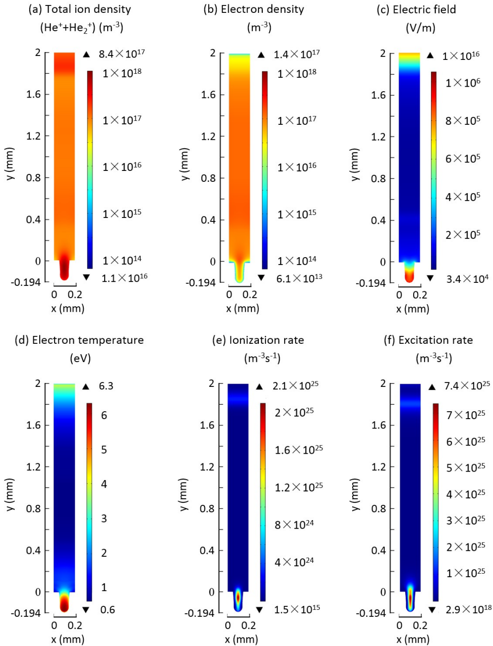
Figure 11: Calculated distributions of the total ion density (a), electron density (b), electric field (c), electron temperature (d), electron impact ionization rate (e) and electron impact excitation rate, averaged over one period, as obtained from fluid modeling for a helium DBD with applied voltage of 20 kV, and with a 100\ \mu\text{m} pore at the bottom dielectric (with dielectric constant of 9) [45]. Note that in (a) and (b) the same color scale is used, to allow comparison, but the values above and below the
