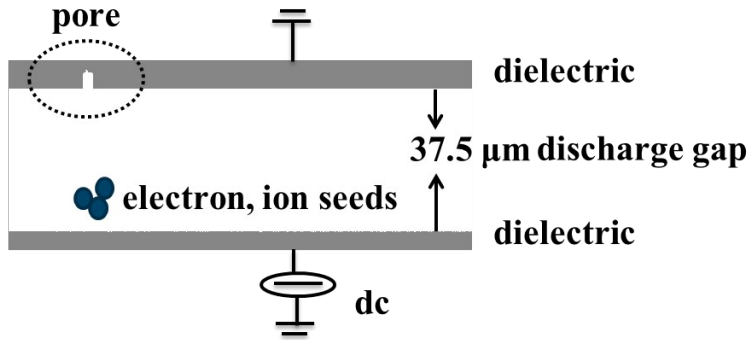
Figure 2: Schematic illustration of the simulation geometry for modeling the behavior of plasma streamers in catalyst pores in a DBD reactor, by 2D PIC/MCC simulations.
