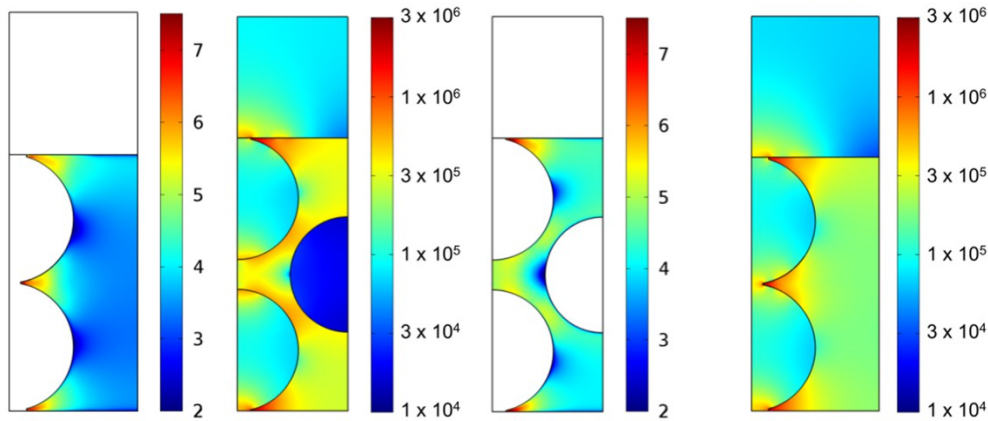
Figure 3: Calculated time-averaged electric field ( E ; a,b) and electron temperature ( T_e ; c,d) in a packed bed DBD reactor in helium, obtained from two complementary 2D fluid models [29], to mimic best the real 3D geometry, i.e., with two beads in contact with each other (so-called “contact point” model) (a,c), and with three beads, not entirely in contact with each other, allowing a channel of voids where the gas can pass through (so-called “channel of voids” model) (b,d), at a peak-to-peak voltage of 4 kV and a frequency of 23.5 kHz.
