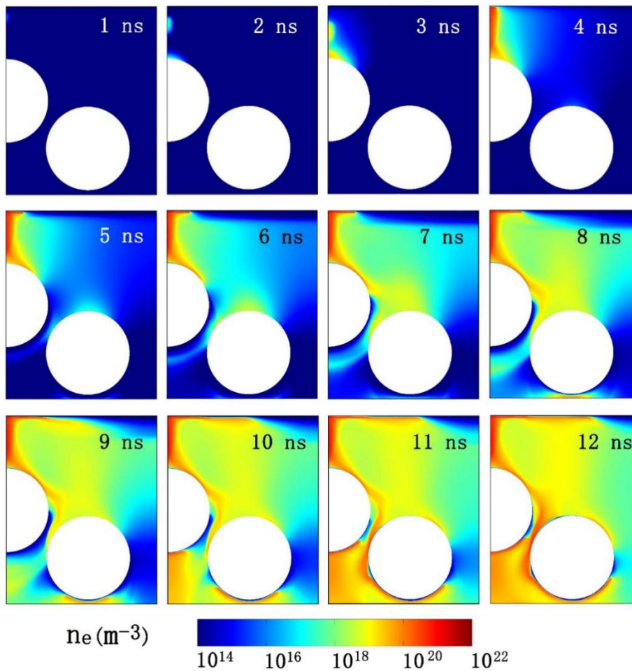
Figure 7: Calculated electron number density evolution as a function of time, as obtained with a fluid model, for a packed bed DBD reactor in dry air, with two packing beads of \epsilon_r = 5 , and applied voltage of -10 kV at the top electrode. Adopted from [32] with permission.
