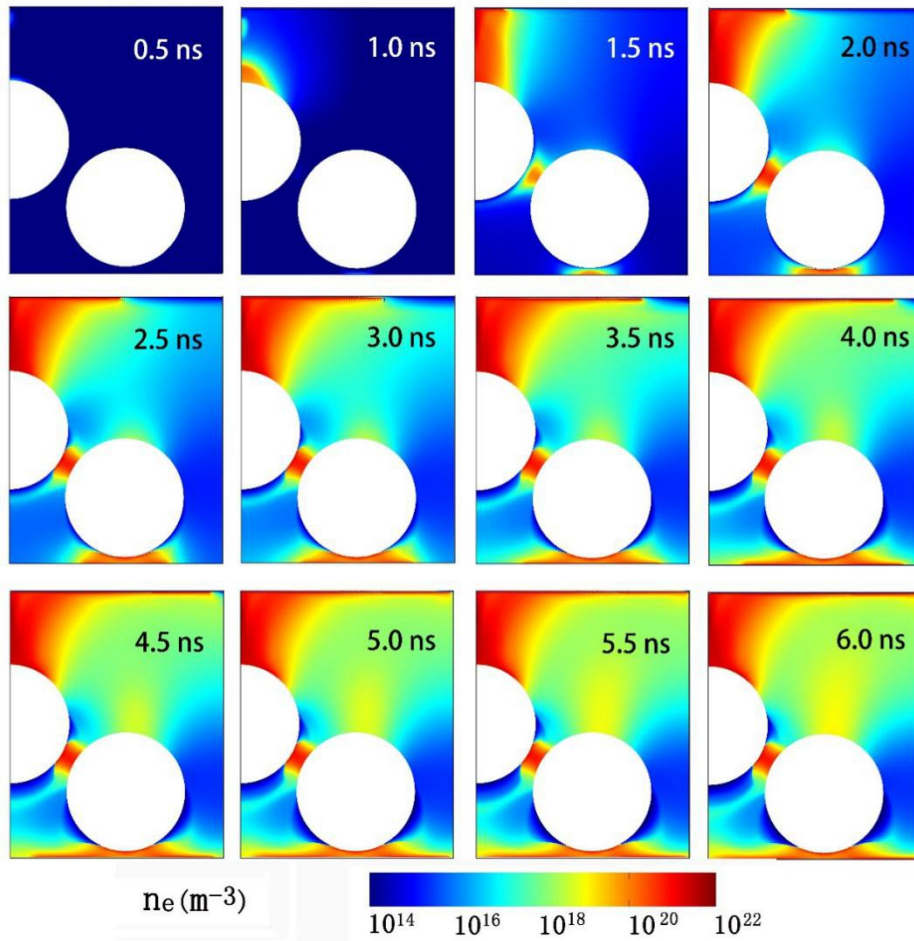
Figure 8: Calculated electron number density evolution as a function of time, as obtained with a fluid model, for a packed bed DBD reactor in dry air, with two packing beads of \epsilon_r = 1000 , and applied voltage of -10 kV at the top electrode,. Adopted from [32] with permission.
