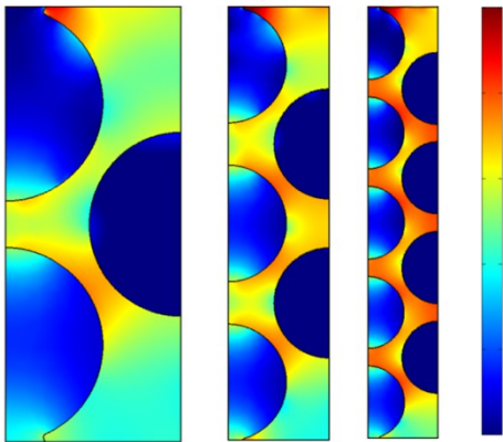
Figure 5: Calculated time-averaged electric field strength for a packed bed DBD reactor in helium, with 3, 5 and 9 beads, with dielectric constant of 1000 ( \sim BaTiO 3 packing), as obtained with a fluid model [31]. The gap size is 4.5 mm, and the applied voltage is 7.5 kV (peak-to-peak).
