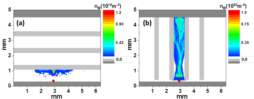
Figure 9: Calculated electron number density profile ( \text{m}^{-3} ), illustrating the formation of a plasma streamer in a DBD reactor in dry air, with honeycomb monolith structure with channels parallel (a) and perpendicular (b) to the electrodes, as obtained from PIC/MCC simulations [35]. The red spot indicates the location of the seed particles (i.e., where the streamer is initiated). The dielectric plates covering the electrodes are depicted in dark grey colour, while the honeycomb structure is in light grey colour.
