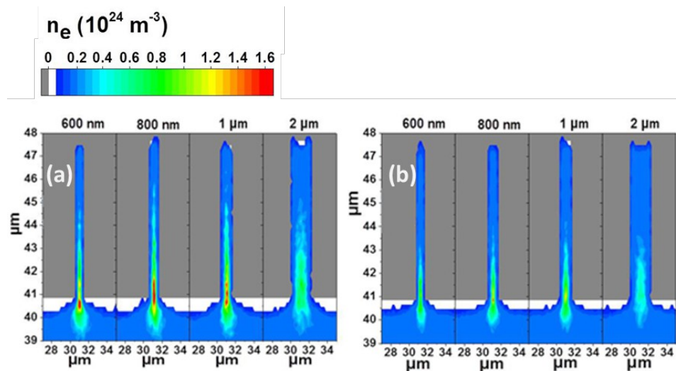
Figure 13: Calculated electron density profile, in m^{-3} , near and inside a pore with diameter of 600 \text{ nm} , 800 \text{ nm} , 1 \mu m , and 2 \mu m , for \epsilon_r = 25 (a), and \epsilon_r = 200 (b), as obtained from PIC/MCC simulations in dry air, for an applied DC voltage of -8 \text{ kV} [50].
