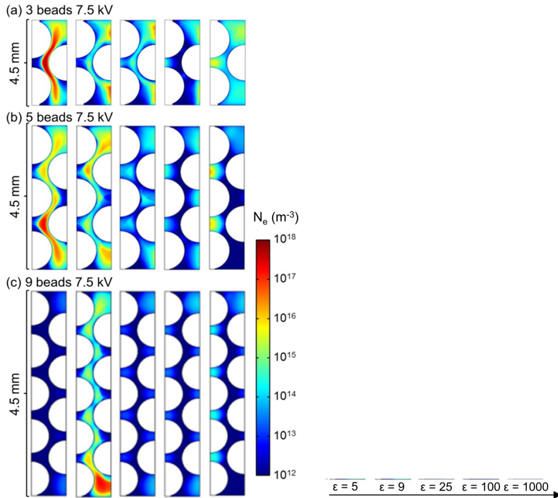
Figure 6: Calculated time-averaged electron density profiles for a packed bed DBD reactor in helium, with 3, 5 and 9 beads, for different dielectric constants, as obtained with a fluid model [31]. Note that the different geometries have the same actual gap size (4.5 mm), but it was enlarged for the smaller bead sizes, to better visualize the behavior.
