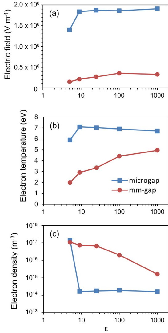
Figure 4: Calculated space- and time-averaged electric field strength (a), electron temperature (b), and electron density (c), as a function of the dielectric constant of the packing beads ( \epsilon ), obtained with a fluid model in helium, for both a microgap (500 \mu\text{m} ) and a mm-gap (4.5 mm) packed bed DBD reactor, with the same applied voltage of 7.5 kV (peak-to-peak). Reproduced with permission from [30].
