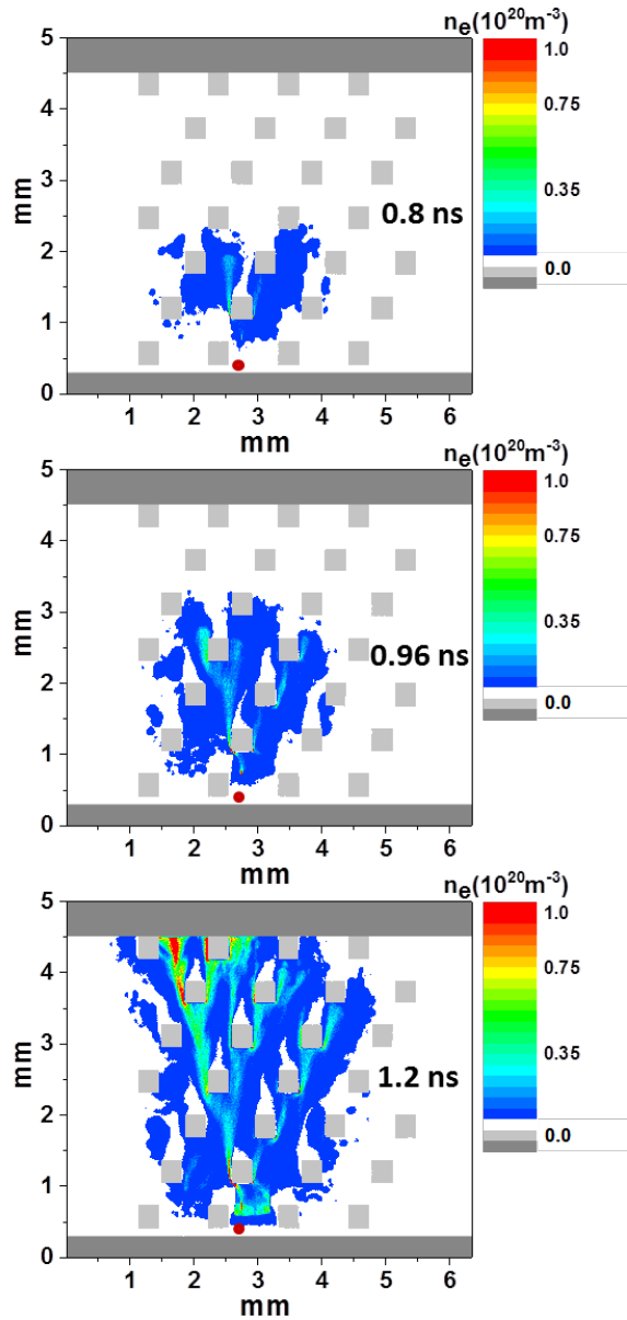
Figure 10: Calculated electron number density profile ( m^{-3} ), at different times, illustrating the evolution of a plasma streamer in a DBD reactor in dry air, with 3DFD 1-3-5 stacking architecture, as obtained from PIC/MCC simulations [35]. The red spot indicates the location of the seed particles (i.e., where the streamer is initiated). The dielectric plates covering the electrodes are depicted in dark grey color, while the fibers of the 3DFD structure are in light grey color. It is clear that the streamers can distribute to different channels, yielding a broad plasma distribution.
