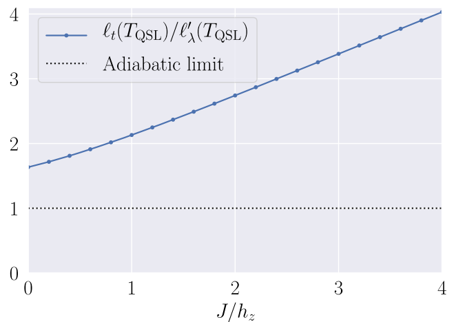
FIG. 1. Numerical justification of the conjecture (2), at the quantum speed limit of preparing the interacting ground state of H_{3\text{LS}} with the noninteracting fast-forward Hamiltonian H_{2\text{LS}}(t) . The parameters are \lambda_i/g = -2 = -\lambda_*/g .
