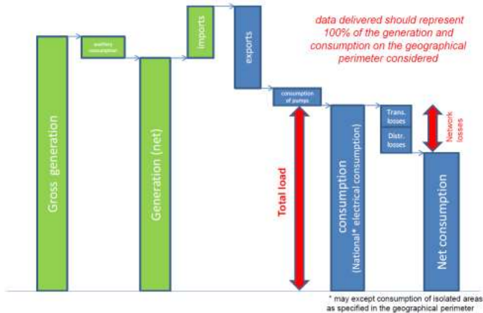
Fig. 1 definition of generation, consumption and load (Data Expert Group ENTSO-E 2015)
