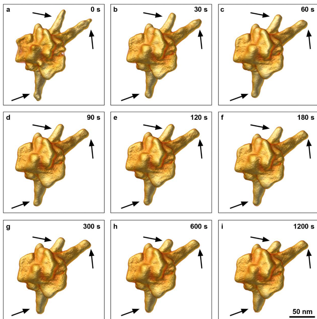
Figure 2. 3D visualizations of the same Au NS after different heating times at 200 °C. The black arrows point towards the regions where morphological changes can be clearly seen.
