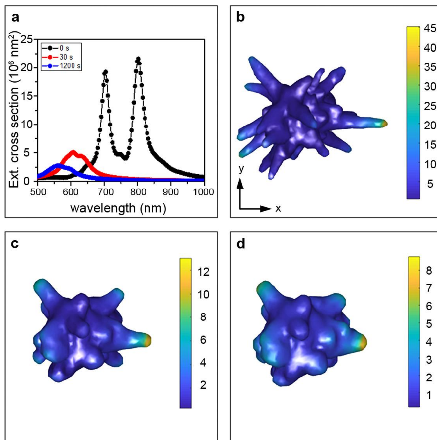
Figure 6. BEM simulations of the Au NS heated at 300 °C, performed on a simplified surface deduced from the corresponding 3D tomographic reconstructions. (a) Extinction cross sections for the unheated and heated NS, after 30 s and 1200 s of heating at 300°C. The calculated average induced electric field is shown for the unheated NS (b), after heating for 30 s at 300 °C (c) and after heating for 1200 s at 300 °C (d).
