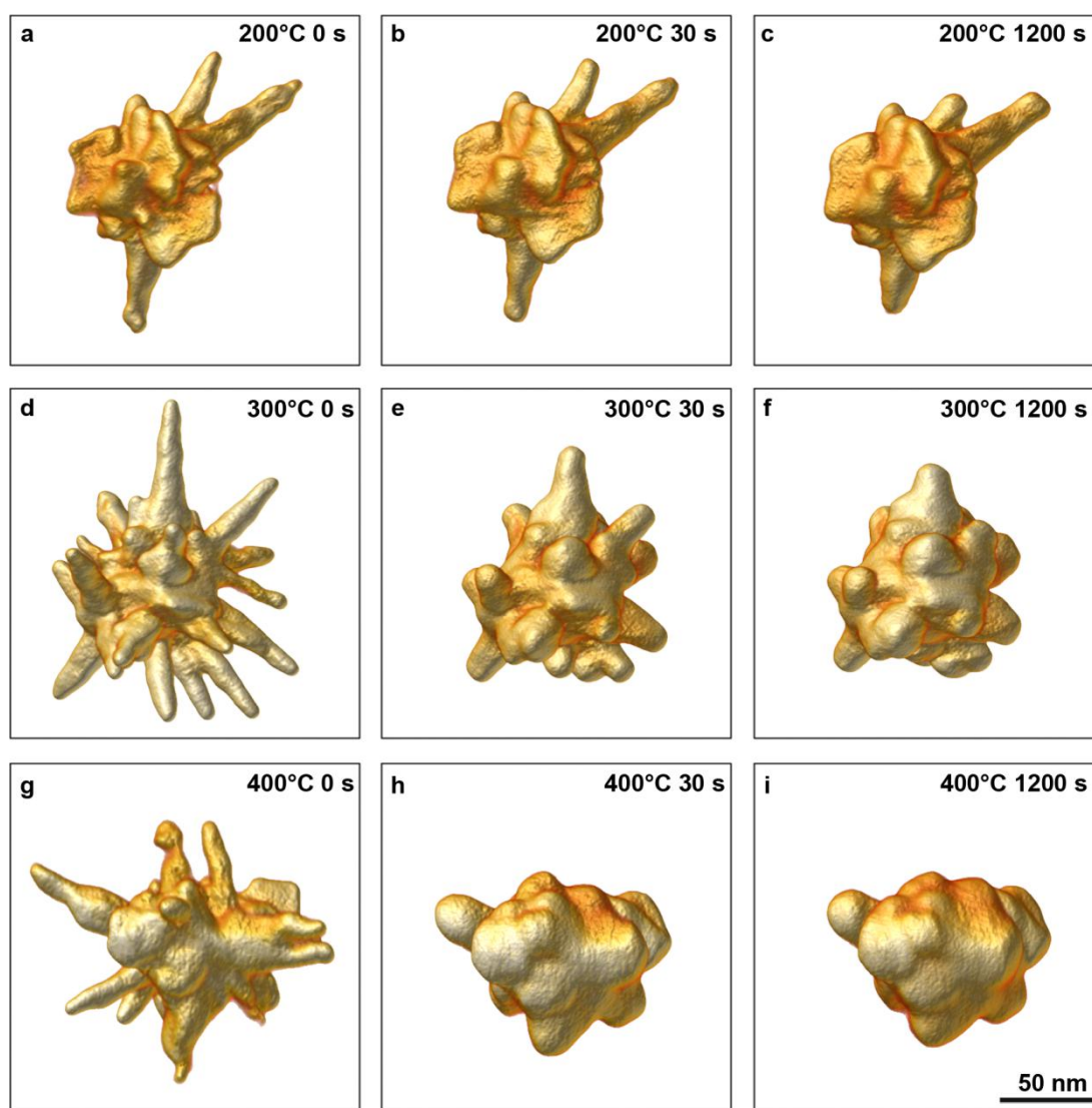
Figure 3. 3D visualizations, using fast tomography, of an Au NS before (a) and after heating for 30 s (b) and 1200 s (c) at 200 °C. 3D visualizations for the same time steps are shown for 300 °C (d-f) and 400 °C (g-i).
