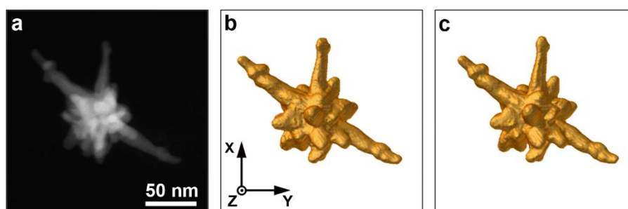
Figure 1. (a) 2D HAADF-STEM image of an Au NS. (b, c) 3D visualizations of the outcome of the conventional tomography experiment (b) and the fast tomography experiment (c).
