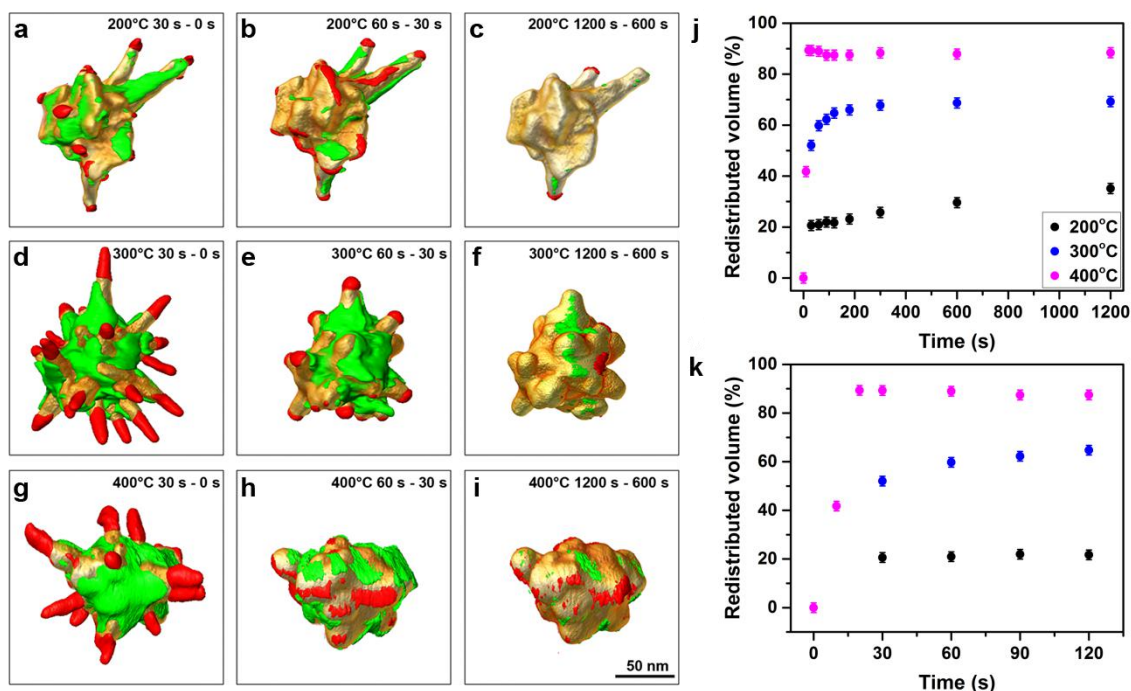
Figure 4. (a-i) Visualizations of the morphological changes during two successive heating steps, where volume increments and volume reductions are depicted in green and red, respectively. The order of subtraction is indicated in each panel, together with the temperature of heating. (j) Total amount of redistributed volume normalized to the volume of the branches in the initial NS, as a function of time for 200 °C (black dots), 300 °C (blue dots) and 400 °C (magenta dots). (k) Detailed view of the volume redistribution occurring during the first two minutes.
