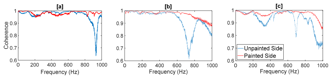
Figure 5. Coherence function of the specimens: (a) thin asphalt layer (TAL); (b) poroelastic road surface (PERS); (c) stone mastic asphalt (SMA).
