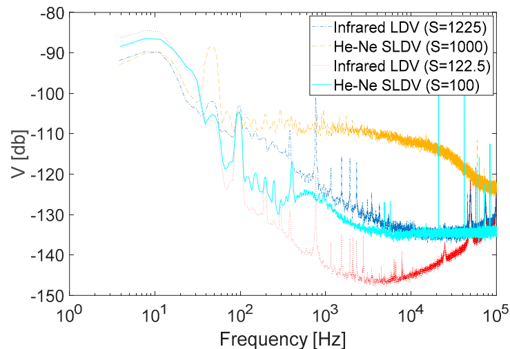
Figure 3. Noise floor comparison between He-Ne and infrared laser Doppler vibrometer (LDV); S = sensitivity (mm/s/v).
