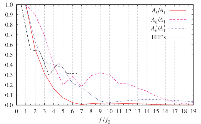
Figure 8. Amplitude ratios, A_k/A_1 , A_k^-/A_1^- , A_k^+/A_1^+ and amplitude of the half-integer frequencies, plotted versus the frequency (harmonic orders indicated by vertical dashed lines). Results for the model of set M6 with T_{\text{eff}}^s = 6800 K.
