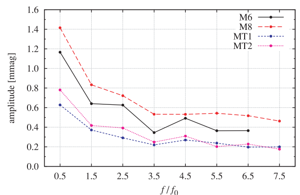
Figure 11. Amplitudes of half-integer frequencies for models of sets M6, M8, MT1 and MT2 (initial non-modulated model was the same for all four models displayed, and its effective temperature was 6800 K).
