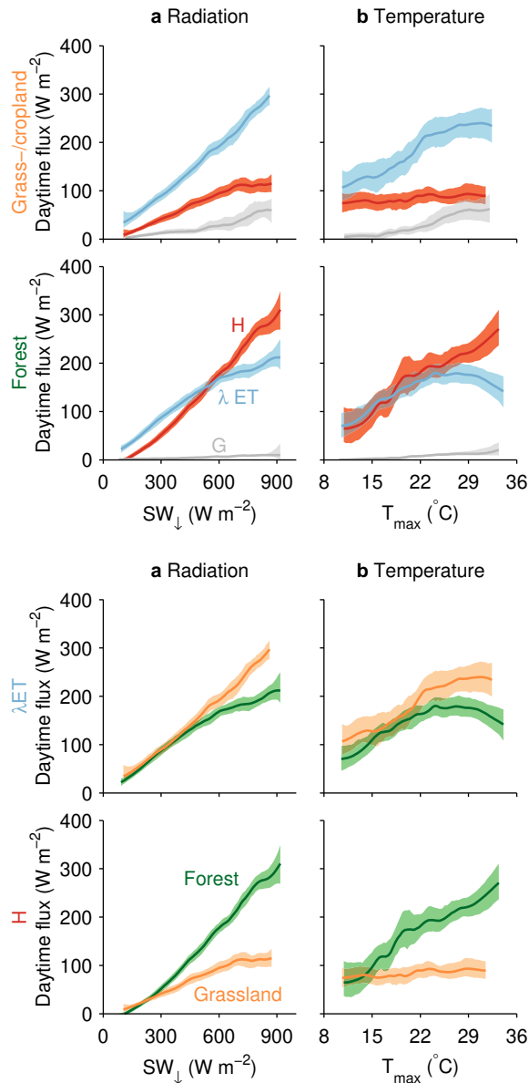
Supplementary Figure 2 | Functional relationships between midday surface fluxes of sensible heat ( H ), latent heat ( \lambda ET ), and ground heat ( G ) and environmental conditions. a , Incoming shortwave radiation ( SW_{\downarrow} ). b , Daily maximum air temperature ( T_{\max} , see Supplementary Table 1 for non-heatwave site averages). Curves have been derived using locally weighted polynomial regression (LOESS) on all midday data (9:00–13:00 UTC, heatwave days included) in the months June–August for all sites. Uncertainty bounds reflect 5% and 95% percentiles of the LOESS regression as determined by bootstrapping. The upper plot displays the relations per land use type separately; in the lower plot the relations are shown for H and \lambda ET separately. Relationships with radiation are stronger than with temperature as indicated by the smaller uncertainty bounds. Note that grassland and forest have different maxima in their T, \lambda ET -relationships, with forest becoming temperature limited at lower temperatures. The sensible heat flux over grassland shows no clear relation with temperature over the observed range of temperatures, whereas it strongly increases with temperature over forest.
