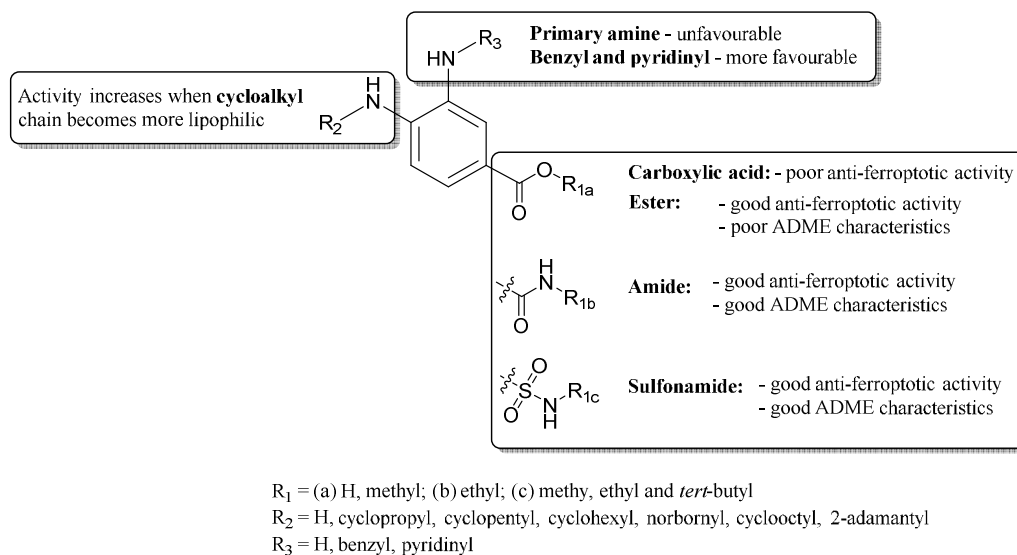
Figure 5. General structure-activity relationship (SAR) from combining anti-ferroptotic activity and the results from the ADME assays.
