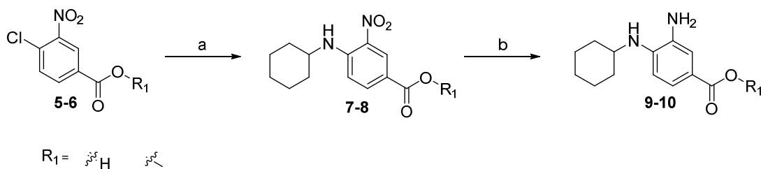
Scheme 1: Reagents and conditions: (a) cyclohexylamine, K_2CO_3 , DMSO, 17h, 60^\circ C ; (b) Palladium hydroxide, H_2 gas, methanol, 17h, rt;
