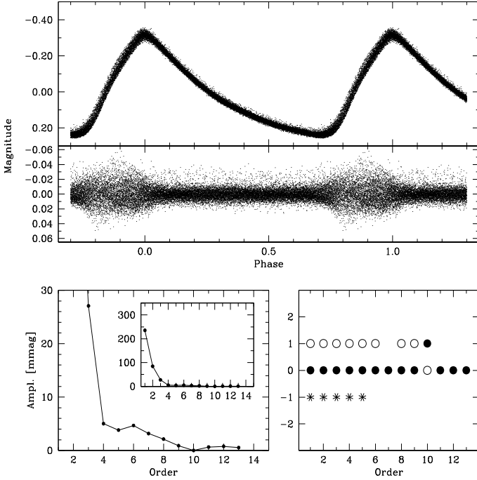
Fig. 3. Upper panel: the CoRoT data folded with f_0 , original (top) and after subtracting the 79 frequencies (bottom). Left panel, lower row: the amplitudes of the n f_0 terms. Right panel, lower row: the observed triplet structure around n f_0 terms. The filled circles indicate the component with the greatest amplitude in the triplet, the empty circles the second in amplitude, the star the third.
