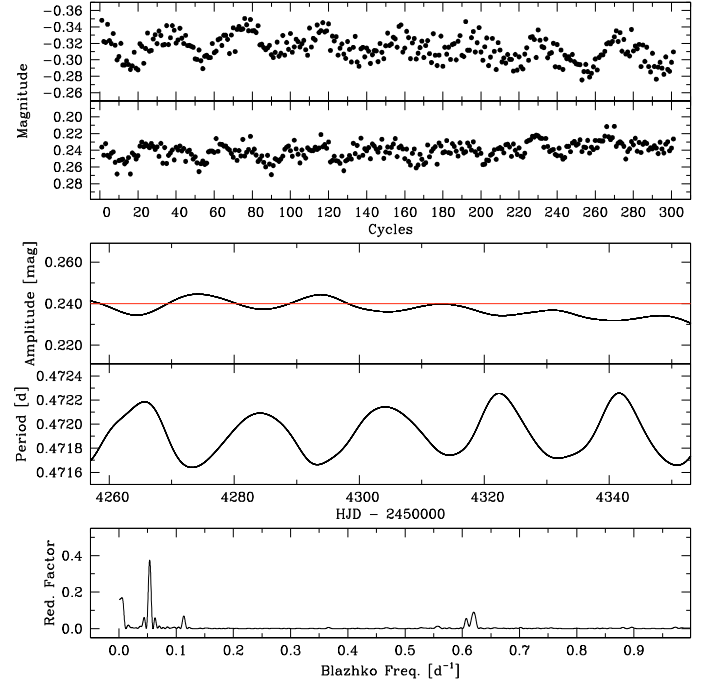
Fig. 4. Evidence of the long-term variations in the CoRoT 101128793 light curve. Top panel: the magnitudes at maximum (upper curve) and minimum (lower curve) brightness in the different cycles. Middle panel: the amplitudes of the f_0 component (upper curve) and the period values (lower curve). Reference line is displayed to show the long term variation in amplitude. Bottom panel: the power spectrum of the magnitudes at maximum brightness.
