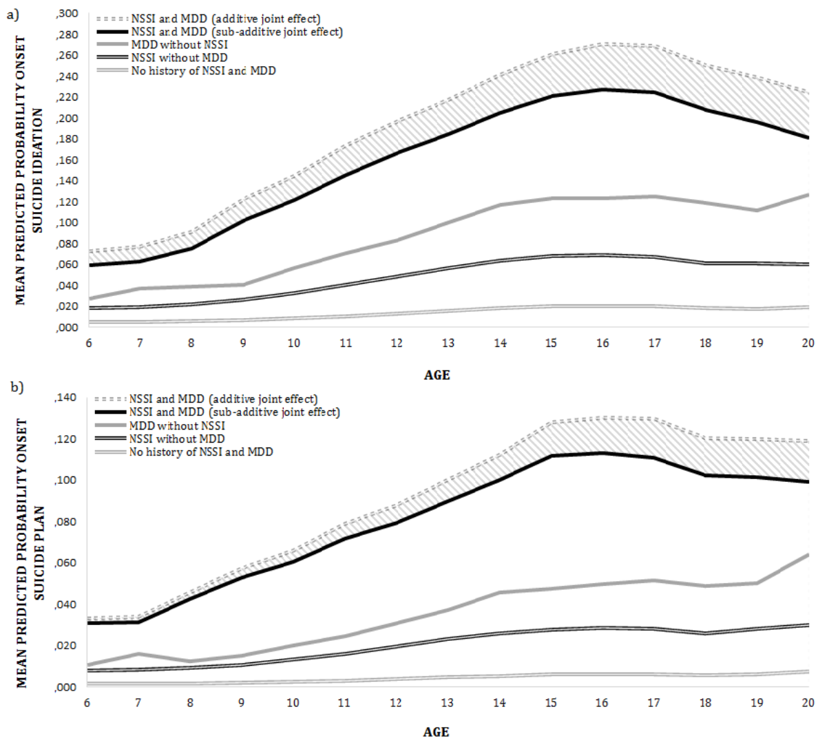
Figure 1. Mean Predicted probability curves for an onset of suicide ideation (a) and suicide plan (b) a
