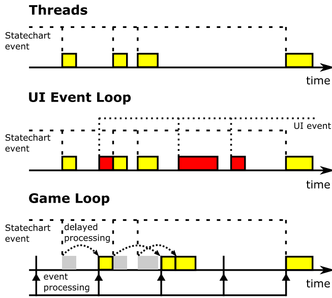
Figure 3. The three runtime platforms.
