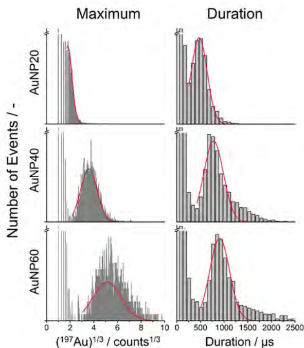
Figure 1: Frequency distributions of maximum intensity and event duration obtained for three different sizes of AuNPs as example. Data of maximum intensity is plotted as cubic root, to account for the cubic relation of particle volume or mass, and diameter allowing to apply a linear Gaussian fit (red line). The left-sided, not fitted bars are contributions of the background noise. All horizontal axes share the same scale in one column.
