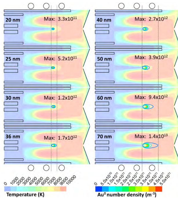
Figure 6: 2D-profiles of atomic Au number density for AuNPs of different diameters. The maximum densities (in m -3 ) are also indicated. For comparison, the plasma temperature contour lines are also plotted in faint colors, showing that the temperature profile is not affected by the NP introduction. The vertical dashed lines indicate the atomic cloud length for the AuNPs of 36 nm (left panels) and 70 nm (right panels), indicating that the atomic cloud extends over a wider region for the larger NPs.
