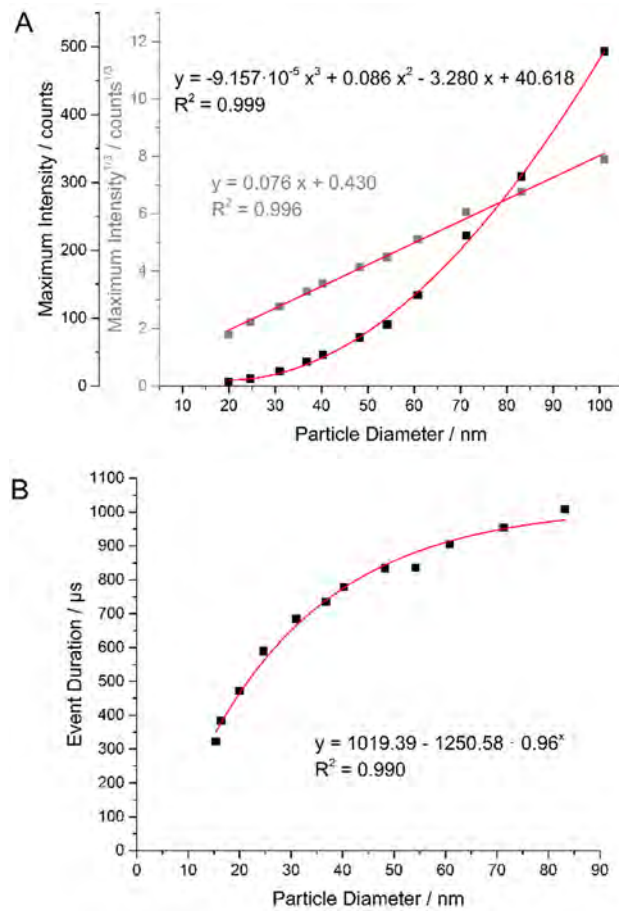
Figure 2: Means of Gaussian fit obtained from the frequency distributions of each particle suspension, for the maximum intensity (A) and event duration (B) versus particle diameter as obtained from TEM analysis. In (A), the cubic root of maximum intensity is also plotted (grey data points and grey y-axes), showing a linear relationship with particle diameter, and thus confirming the cubic relationship of particle volume or mass versus particle diameter.
