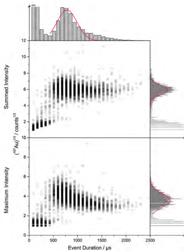
Figure 3: 2D-visualization of all three single particle event characteristics for AuNP40. Each square represents one single particle event and is placed in the 2D-plot either for its summed intensity and event duration (upper section) or maximum intensity and event duration (lower section). The squares are plotted in a transparent way, so that areas of more frequent event characteristics appear darker, which is also indicated by the histograms of summed and maximum intensity (vertical axes) and event duration (horizontal axis).
