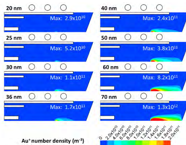
Figure 4: 2D-profiles of \text{Au}^+ number density for AuNPs of different diameters. The maximum densities (in \text{m}^{-3} ) are also indicated. Only half of the 2D axisymmetric torch is plotted.
