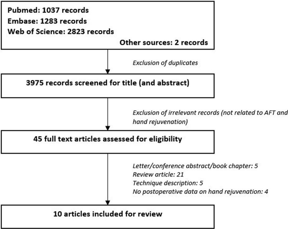
Figure 1. Flow diagram of the search strategy
