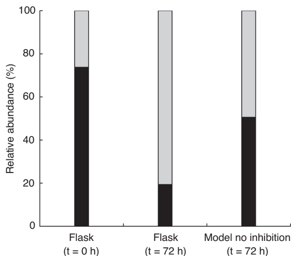
Figure 3 Liquid culture competitive growth experiment showing the relative abundance of Rhodobacter blasticus EBR2 (■) and the Rhodopseudomonas palustris EBE1 (□) at time (t) 0 h, 72 h and through the growth model. The PNSB abundancies in the growth model were calculated using the equation N = N_0 * e^{\mu_{max} * (t_{final} - t_{lag})} without considering competitive inhibition. The abundance was corrected for 16S gene copies per genome.
