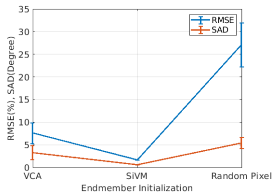
Fig. 19. Comparison of different endmember initializations for HapkeCNN. The performance is given in terms of SAD in degree and RMSE in percentage. The experiments were performed on the simulated dataset 2 (30 dB).
