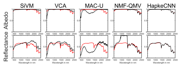
Fig. 20. Endmember 6 of simulated dataset 2 (40dB) - Visual comparison of the albedo and reflectance endmembers by the different unmixing techniques. Red: ground truth endmembers; Black: estimated endmembers.
