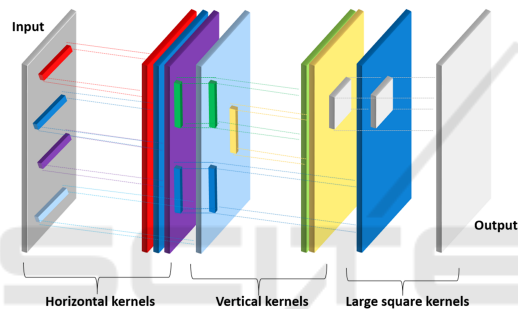
Figure 3: THzNet-2D architecture.
