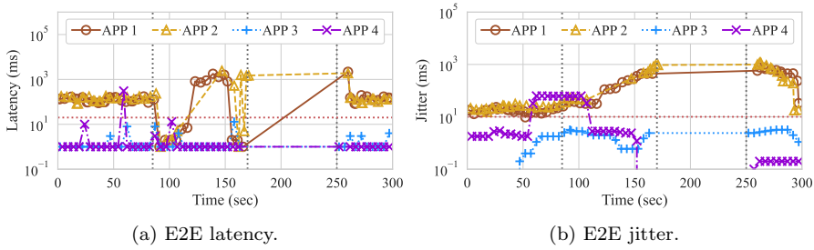
Fig. 9: Experiment 1 E2E latency and jitter of applications.
