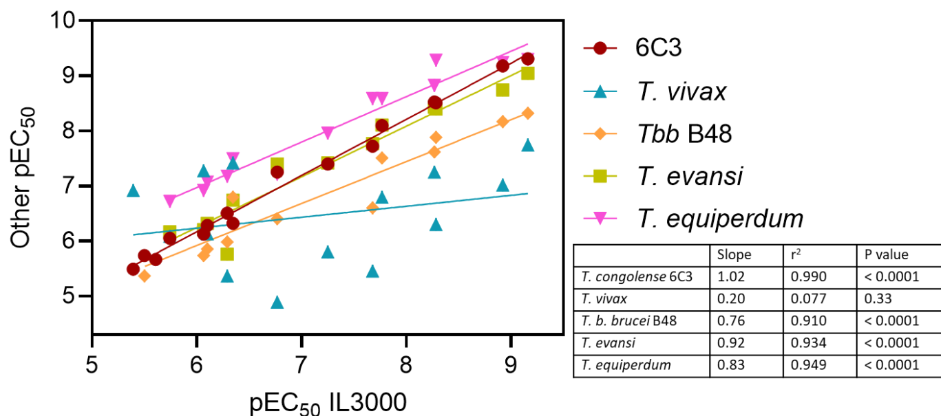
Figure 9. Correlation between the -\log(\text{EC}_{50}) (pEC 50 ) of adenosine antimetabolites against T. congolense IL3000 with the pEC 50 for other Trypanosoma cell lines or species. Lines were obtained by linear regression and slopes, correlation coefficients and p value for slope being non-zero were calculated by GraphPad Prism v8.
