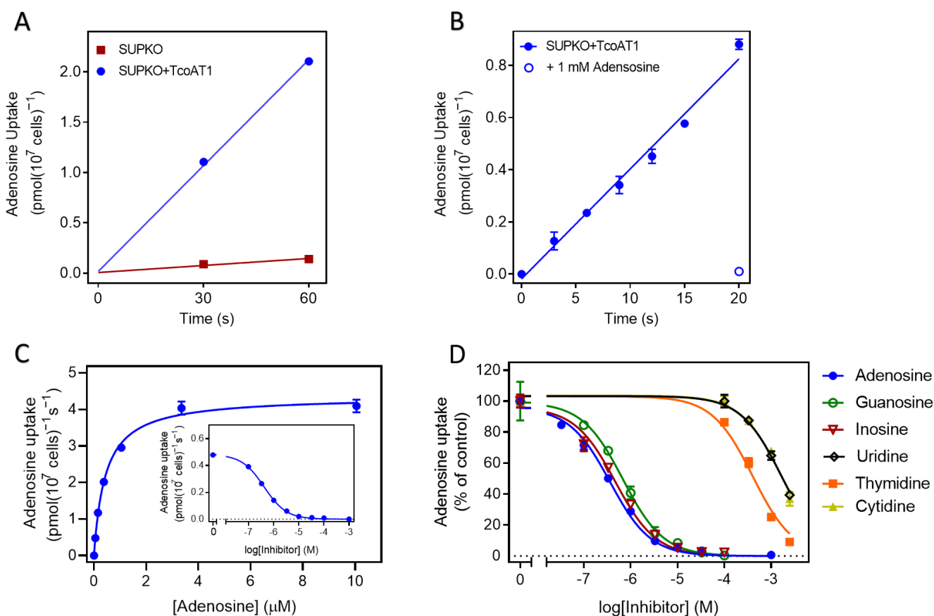
Figure 3. Uptake of 0.05 μM [ 3 H]-adenosine in L. mexicana SUPKO expressing TcoAT1. (A) Uptake in L. mexicana SUPKO and SUPKO+TcoAT1 over 60 s. The expression of TcoAT1 restored adenosine uptake in SUPKO. Data represent averages ± SEM of triplicate determinations. (B) Uptake of [ 3 H]-adenosine in L. mexicana SUPKO+TcoAT1 within linear phase of 20 s. (C) Adenosine uptake by SUPKO+TcoAT1 in the presence of 0–1 mM unlabeled adenosine. Graph shows one representative out of three independent experiments carried out in triplicate all showing a similar result. (D) Substrate specificity of TcoAT1 determined by uptake assays. TcoAT1 has high affinity for both amino- and oxopurines. Inhibition constants ( K_i ) for purines were lower than those of pyrimidines. Adenosine uptake is presented as percentage of no-inhibitor control. Figure shows one representative out of three independent experiments carried out in triplicate (% adenosine uptake average ± SEM).
