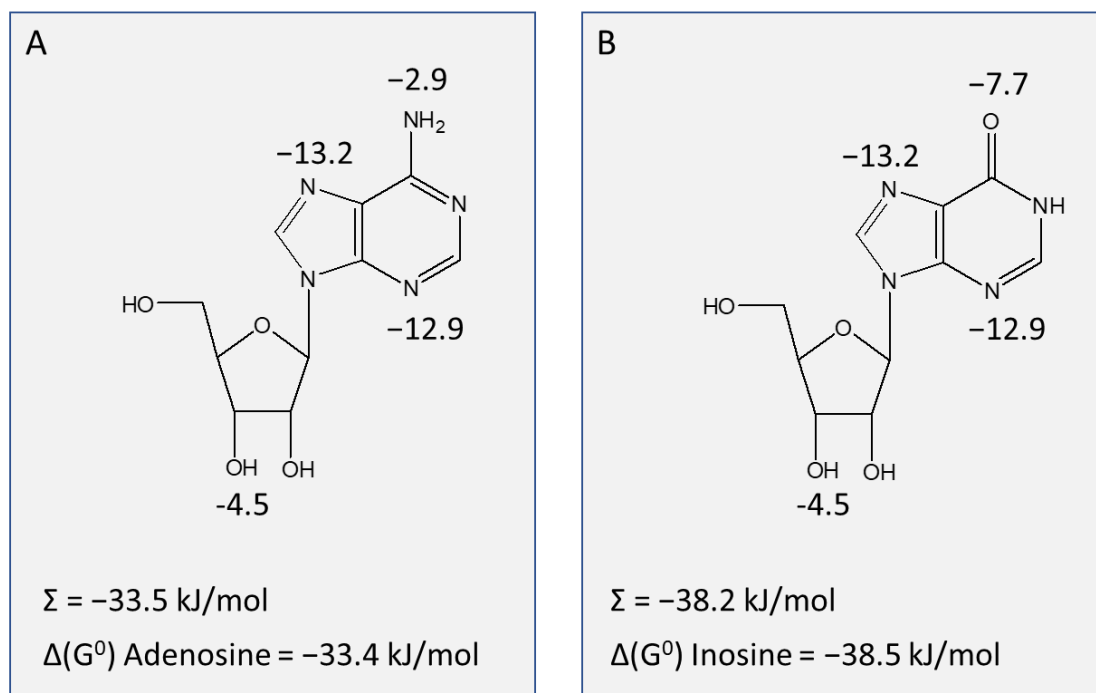
Figure 6. Binding model for TvXNT3 showing points of interaction in adenosine (A) and inosine (B), with the Gibbs free energy of the interaction indicated in kJ/mol. The sum of the interactions and the experimental interaction energies are also indicated.
