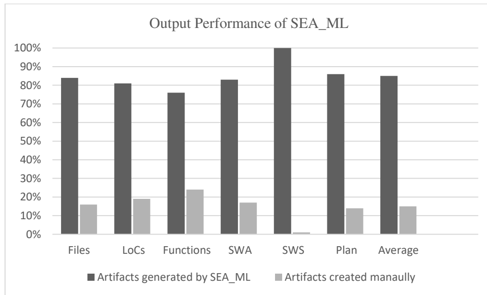
Diagram 1. Output performance of SEA_ML
