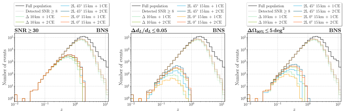
Figure 21. Redshift distribution of detected BNS with \text{SNR} \geq 30 (left column), or relative error on the luminosity distance \Delta d_L/d_L \leq 0.05 (central column), or sky location \Delta\Omega \leq 5 \text{ deg}^2 (right column) for the six 3G the detector networks considered. In each panel, we also show, for reference, the redshift distribution of the BNS population used (black solid line), and of the events detected in the various configurations with \text{SNR} \geq 8 (dotted lines).
