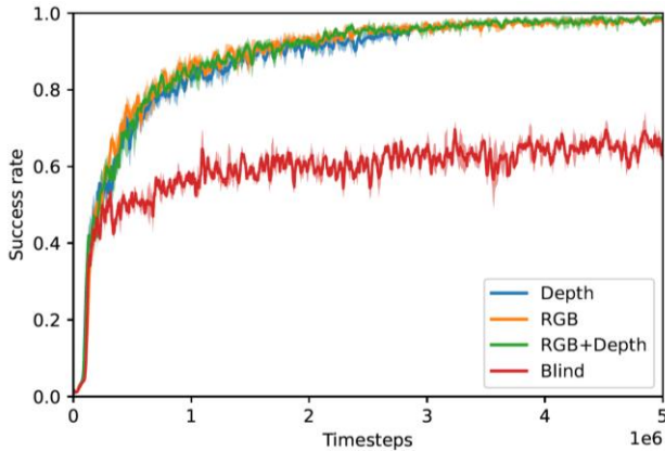
Figure 9. Training performance. The blind agent can perform basic navigation by relying on the GNSS sensor, however to further improve to near perfect results an additional RGB or depth sensor is required to detect and avoid collisions.
