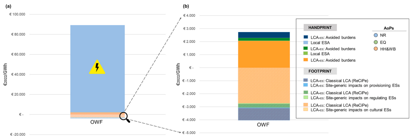
Fig. 7. Quantification of the handprint and footprint of an OWF. The handprint is depicted with colours that have a solid fill, while the footprint have a dashed fill. (a) LCA_{+ES} -ESA results of the OWF (cradle-to-grave), the largest handprint comes from the FU (i.e. local ES wind energy provisioning). Due to the large handprint of the AoP NR, the handprint and footprint of the AoP EQ is not very visible. (b) Handprint and footprint results of the OWF excluding the handprint of the FU. These results comprise the handprint and footprint of LCA_{ES} (i.e. ReCiPe results and site-generic impacts on ESs) and the local marine ESs on each AoP. The impacts on the AoP NR, AoP EQ and AoP HH&WB are depicted in blue, green and orange colours respectively. Most of the handprint of LCA_{+ES} is attributed to the avoided burdens, while the footprint to the ReCiPe results affecting particularly the AoP HH&WB. All the site-generic impacts on ESs are footprints. In Fig. 7b, the handprint value for the local ESA in the AoP EQ (i.e. nursery and habitat maintenance) is below 15 € per GWh, hence cannot be properly visualized. (For interpretation of the references to colour in this figure legend, the reader is referred to the web version of this article.)
