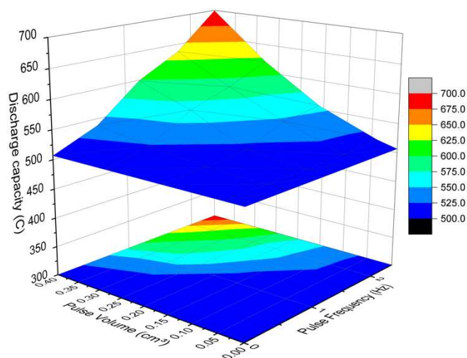
Figure 2. Discharge capacities at a constant current of 100 mA/cm 2 and a constant net flow rate of 5 cm 3 /min as a function of PV and PF.
