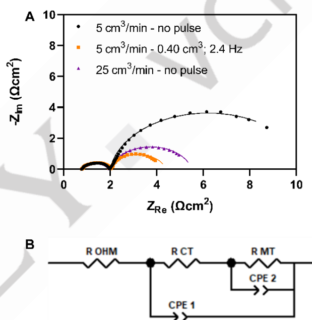
Figure 3. Nyquist plots for a flow rate of 5 cm 3 /min without pulsations, a flow rate of 5 cm 3 /min with pulsations of 0.40 cm 3 PV and 2.4 Hz PF and a flow rate of 25 cm 3 /min without pulsations (A); the electrochemical equivalent circuit (B).
