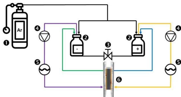
Figure 6. Schematic overview of the experimental arrangement.
