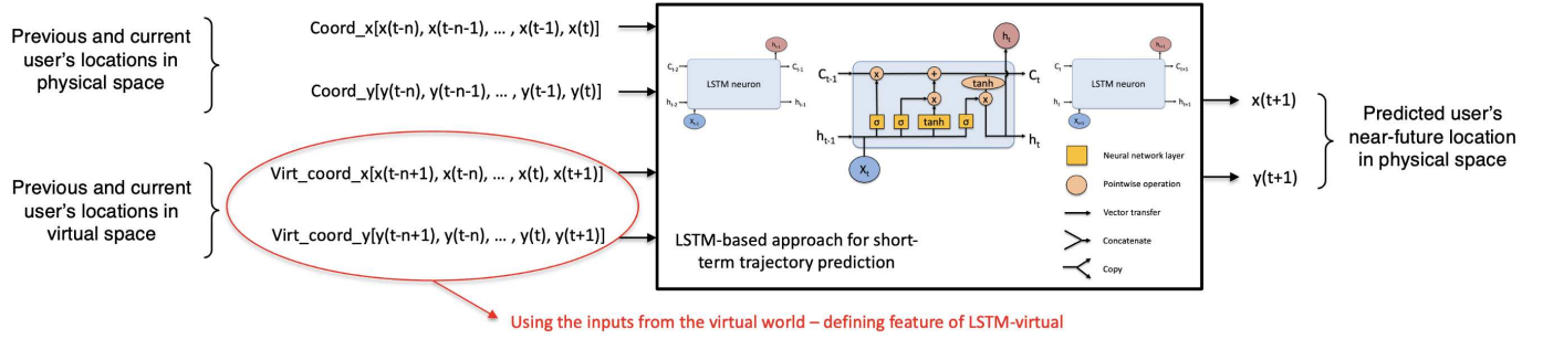
Fig. 2. Input features of the considered LSTM approaches for short-term lateral movement prediction
