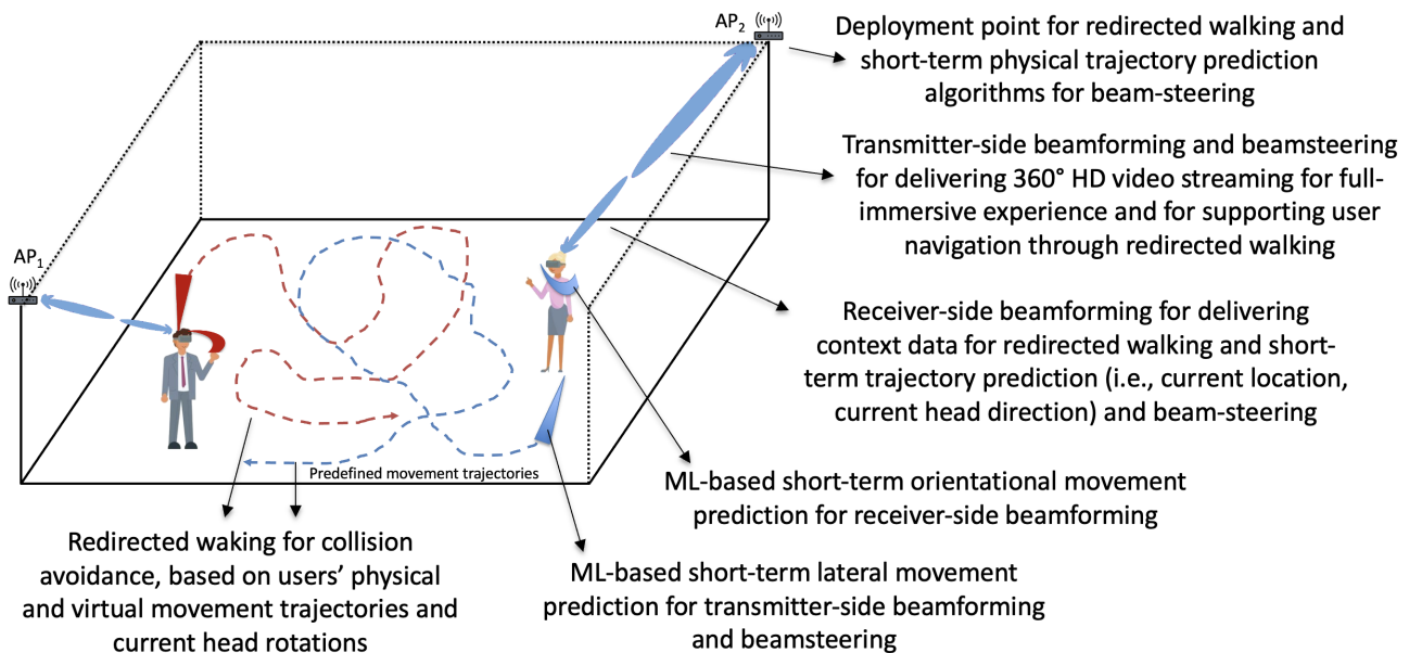
Fig. 1. Considered full-immersive multiuser Virtual Reality setup with Redirected Walking
