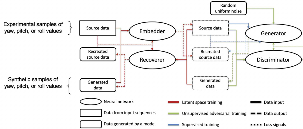
Fig. 3. Proposed design of the TimeGAN-based generation of synthetic orientational movement datasets
