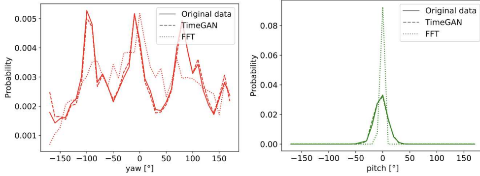
Fig. 5. Yaw and pitch values generated using the considered approaches for generating synthetic orientational datasets
