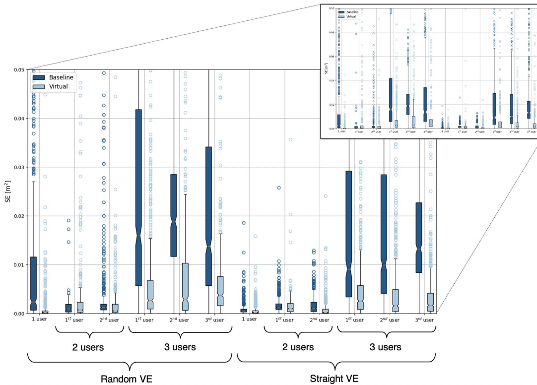
Fig. 4. Squared errors achieved by the considered LSTM-based approaches for short-term lateral movement prediction
