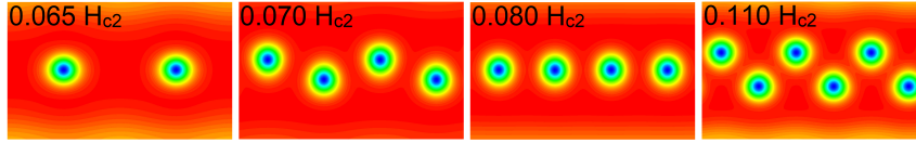
Figure 3.8: Spatial distribution of the superconducting order parameter for a SN of w = 20\xi , at increasing values of magnetic field, shown in each panel in units of H_{c2} . An example of the transition from a single row to a second row, followed by reconfiguration back to a single row due to strong confining effects as a result of the edge Meissner current.
