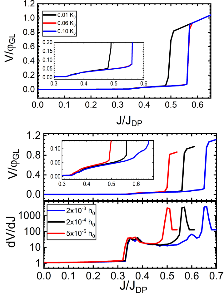
Figure 5.1: Normalised voltage drop as a function of normalised applied current density in units of \varphi_{GL}(T_{bath}) and J_{DP}(T_{bath}) respectively, for a stripe of width w = 19\xi(0) , at applied magnetic field of H = 0.025H_{c2}(0) . Top:- comparison of heat conductivity. Bottom:- comparison of heat transfer, with first derivative of V(J) .
