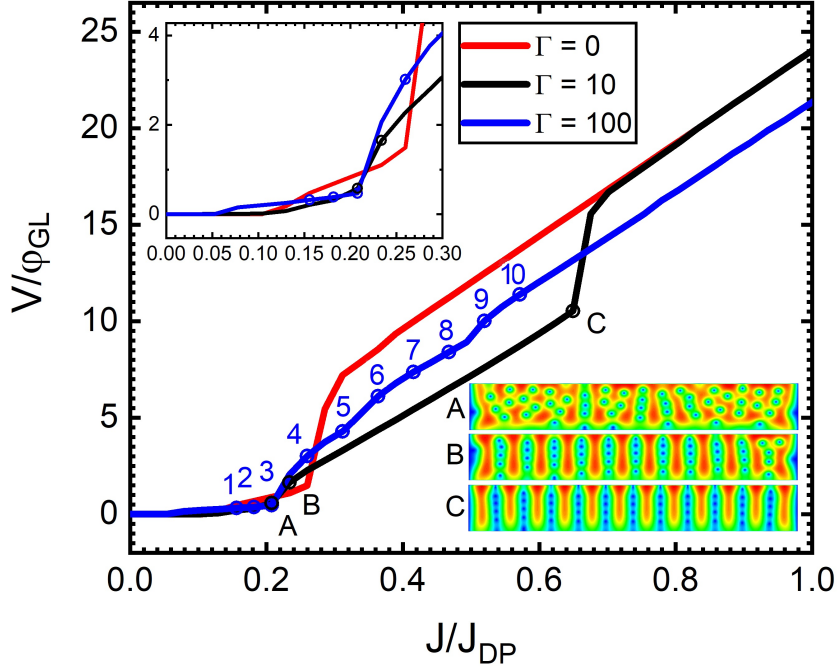
Figure 4.9: Normalised voltage drop as a function of the normalised current density, for a SN of width w = 12\xi , at H = 0.50H_{c2} , and different magnitudes of viscosity \Gamma . The bottom inset shows the spatial distribution of the superconducting order parameter for the stripe with \Gamma = 10 , at different values of J : A: 0.207J_{DP} , B: 0.238J_{DP} , C: 0.650J_{DP} , which are states indicated by back dots on the plot. A zoom of the low J regime, is detailed in the top inset. Blue dots on the \Gamma = 100 profile relate to the snap shots A-J shown in figure 4.10.
