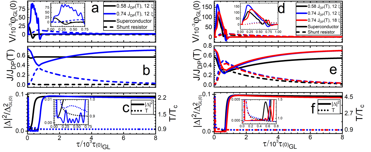
Figure 5.7: Stripe of width w = 38,57\xi(0) , with hot-spot causing a local instantaneous increase in temperature to T_{spot} = 2.2T_c (panels a-c), and T_{spot} = 4.5T_c (panels d-f), with profiles for applied current densities of J = 0.58 and 0.74J_{DP}(0) . Panel a,d - normalised voltage across the stripe as a function of normalised time. Solid line corresponds to the voltage drop across the superconductor, V_s , and the dotted lined corresponds to the potential difference across the shunt resistor, (I - I_s)R_{shunt} . Inset shows zoom of the same profile over the first \sim 1000\tau_{GL}(0) . Panel b,e - normalised current density as a function of normalised time for the current density in the superconductor (solid) and the shunt (dotted). Panel c,f - time dependence of the magnitude of the order parameter (solid) and temperature (dotted) in the center of the hotspot, where the inset shows a zoom of the same profiles over the first \sim 800\tau_{GL}(0) .
