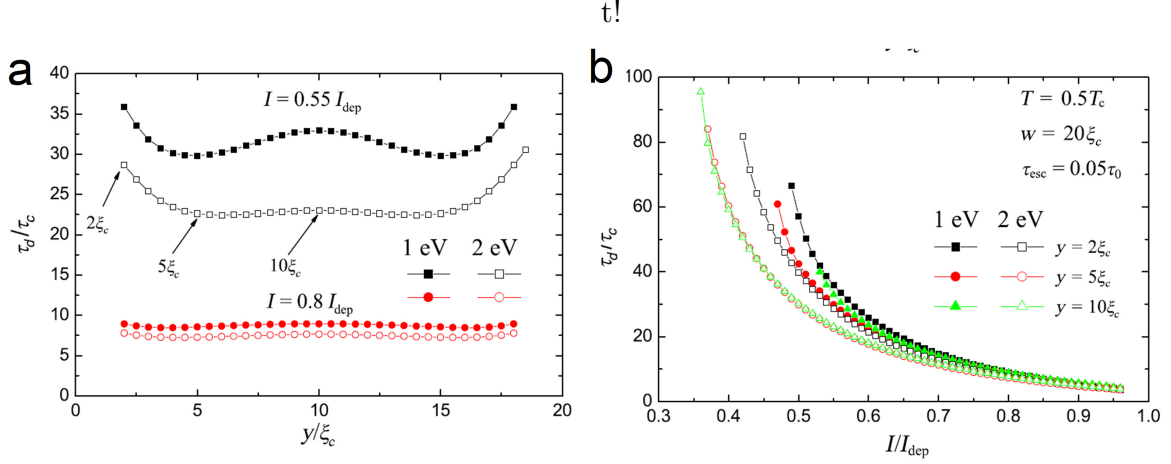
Figure 5.8: Dependencies of the delay time for a stripe of width w = 20\xi , at bath temperature T = 0.5T_c . Panel a- Position-dependent \tau_d at different currents and deposited energies ( E = 1\text{eV} \rightarrow T_{\text{spot}} = 2T_c and E = 2\text{eV} \rightarrow T_{\text{spot}} = 2.4T_c ). Panel b - Dependence of \tau_d on current for three positions of the initial hotspot y = 2, 5, 10\xi and two deposited energies 1 and 2eV. Taken from ref [225] figure 3.
