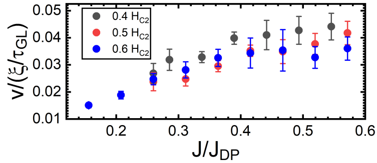
Figure 4.12: Average normalised vortex velocity as a function of the normalised sourced current density for a stripe with \Gamma = 100 , of width 12\xi at applied magnetic fields of 0.4 , 0.5 and 0.6H_{C2} .
