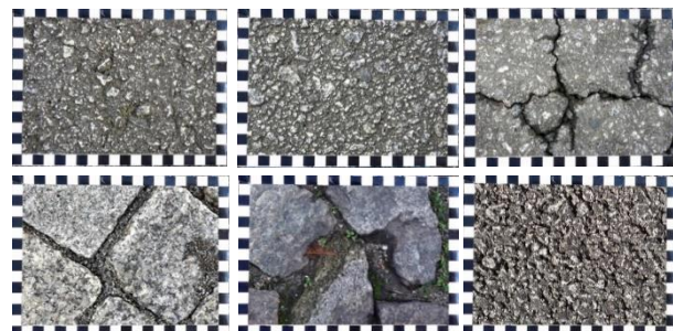
Figure 1. Road surfaces studied. One square in the frame = 1 cm. a) New AC-14; b) 8-years old AC-14; c) AC-14 deteriorated; d) Granite cubes; e) Cobblestones; f) SMA 10 S with RAR X®.
