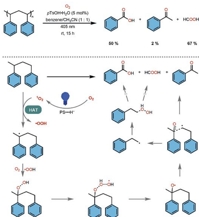
Scheme 5. Acid-catalyzed upcycling of PS.
