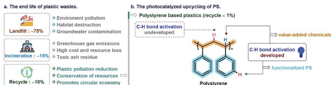
Fig 1. a) The end life of plastic waste. b) The photocatalyzed upcycling of PS.
