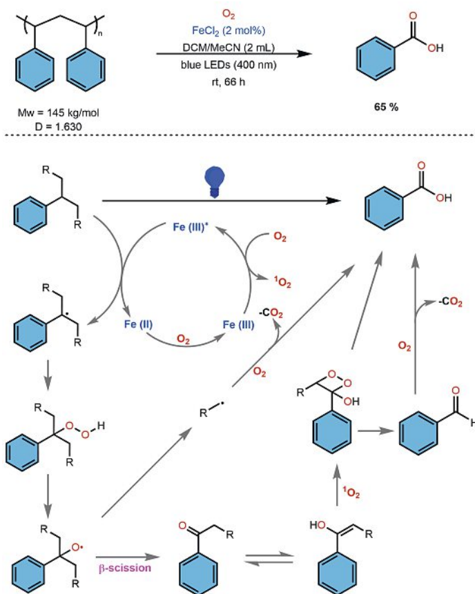
Scheme 3. \text{FeCl}_2 catalyzed upcycling of PS.
