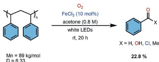
Scheme 4. FeCl 3 catalyzed upcycling of PS with white LEDs.
