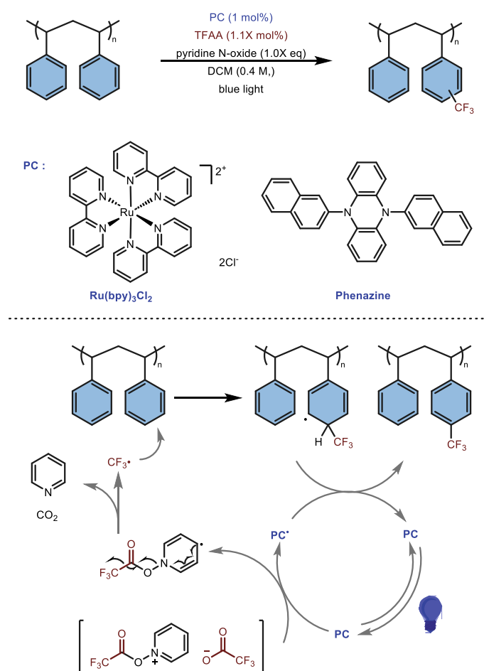
Scheme 1. Photocatalysis PPM of PS.
