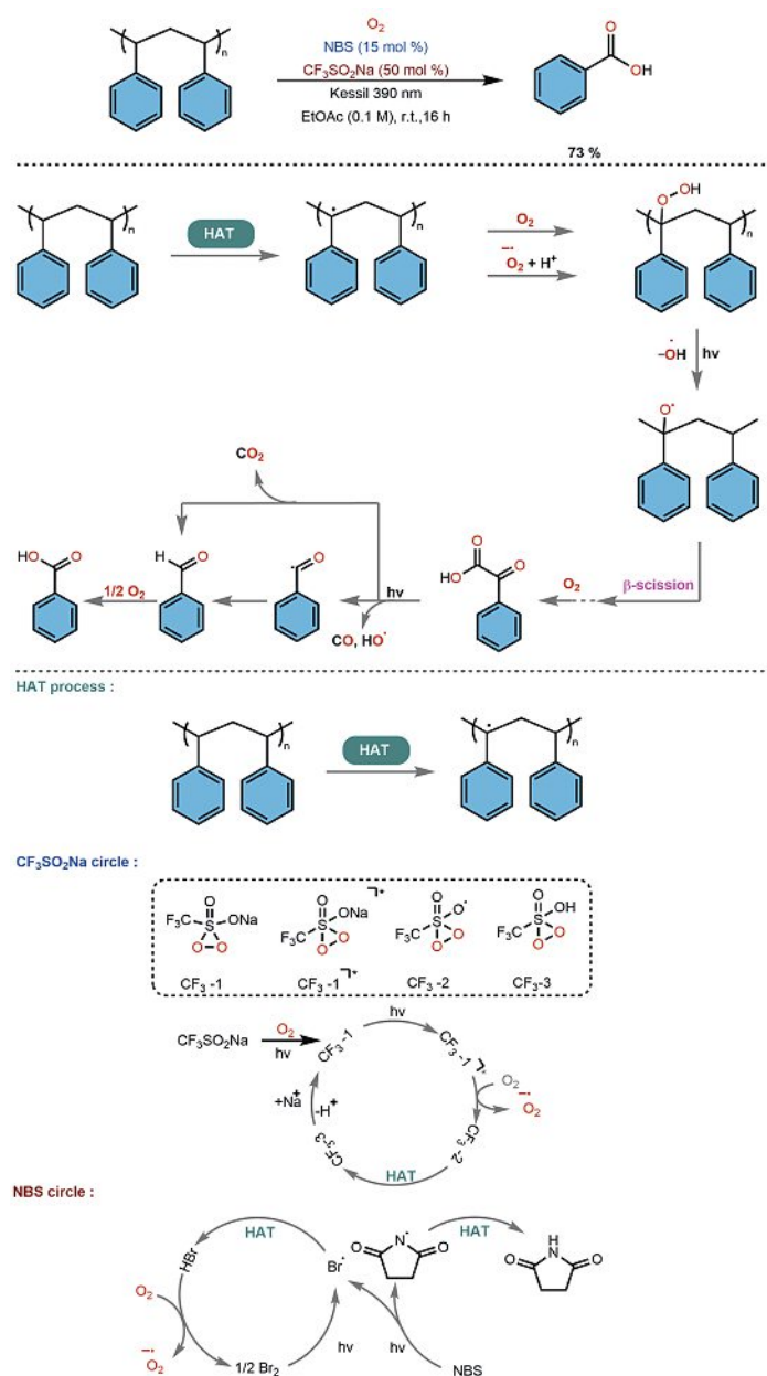
Scheme 6. NBS and CF 3 SO 2 Na catalyzed upcycling of PS.
