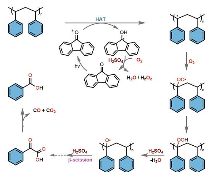
Scheme 7. Fluorenone-catalyzed upcycling of PS.
