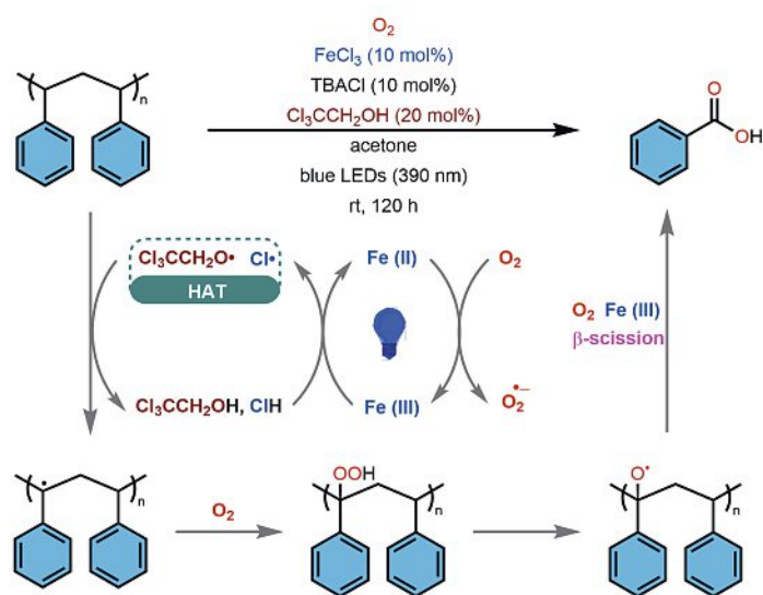
Scheme 2. \text{FeCl}_3 catalyzed upcycling of PS.
