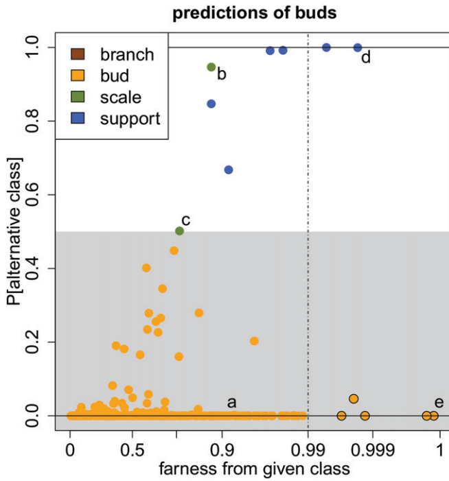
Figure 2. Example of a class map.
