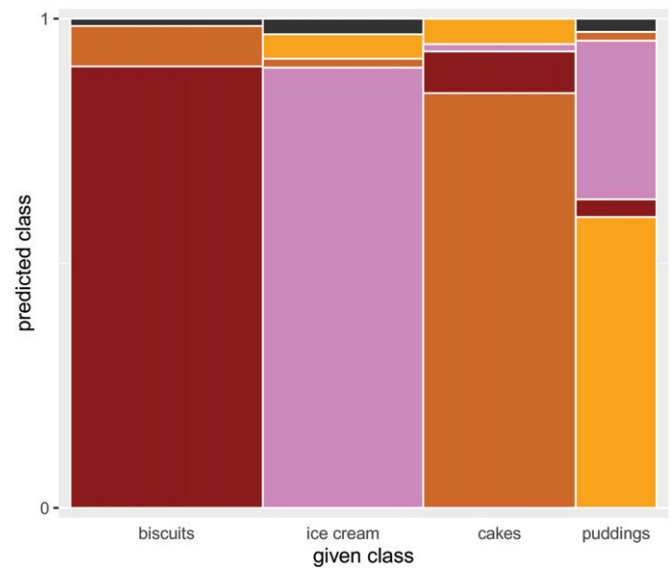
Figure 13. Sweets data: Stacked mosaic plot of the classification. When they occur, the products flagged as outliers are shown in dark gray, as an extra class at the top.
