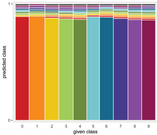
Figure 5. MNIST data: stacked mosaic plot where the objects flagged as outliers are shown in dark gray, as an extra class at the top.
