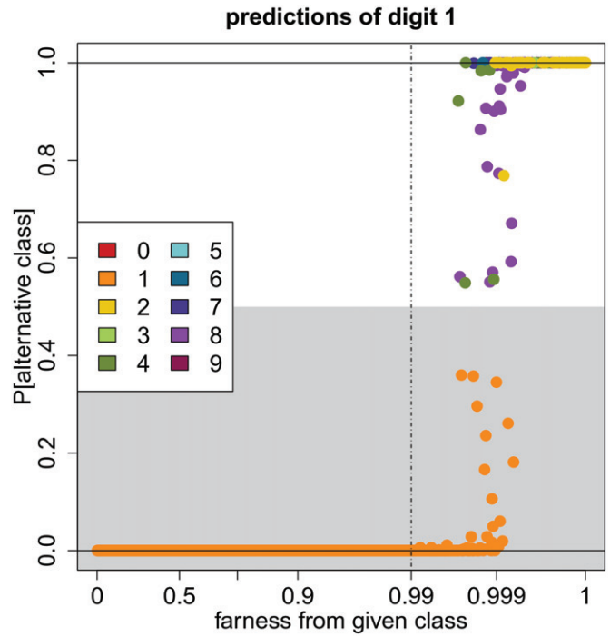
Figure 7. Class map of digit 1.
