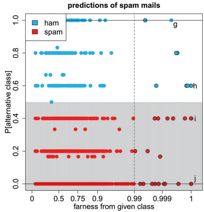
Figure 10. Class map of the spam mails.
