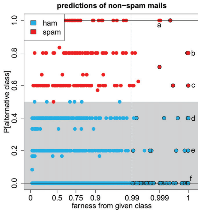
Figure 9. Class map of the nonspam mails.
