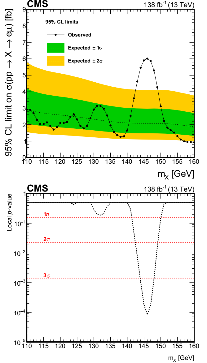
FIG. 7. Upper: the observed (expected) 95% CL upper limits on \sigma(pp \rightarrow X \rightarrow e\mu) as a function of the hypothesized m_\chi assuming the relative SM-like production cross sections of the ggH and VBF production modes. Lower: the observed local p -values against the background-only hypothesis are shown as a function of the hypothesized m_\chi .
