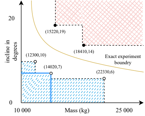
Fig. 3. Experiment map leveraging symbolic reasoning
