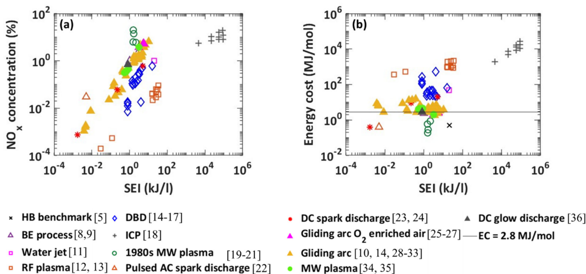
Figure 1. Reported NO x concentration (a) and EC (b) of plasma-based NO x production, as a function of SEI in various plasma reactors. Original references: 1980s low pressure MW plasma, MW plasma at atmospheric pressure, GA, RF plasma, DBD, ICP, spark discharge, and DC glow discharge. The horizontal line in (b) corresponds to the EC of 2.74 MJ/mol, which is the minimum thermodynamic equilibrium EC for atmospheric pressure NF (as discussed further in this paper). Only some low-pressure plasmas produce a lower EC, demonstrating they are characterized by thermodynamic non-equilibrium. Among the atmospheric pressure plasmas (more suitable for upscaling and industrial implementation), warm plasmas, such as GA, MW and DC glow discharge plasmas (all indicated with solid symbols), show the best performance in terms of both NO x concentration and EC (close to the thermodynamic equilibrium limit), as explained in the text.
