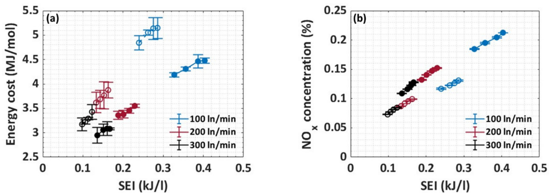
Figure 10. EC (a) and NO x concentration (b) as a function of SEI, for three different flow rates and two distances between the electrodes (dashed lines/open symbols, and solid lines/closed symbols, for d = 7 and 14 cm, respectively), in the large reactor in pin-to-pin configuration. Error bars are indicated but are sometimes too small to be visible.
