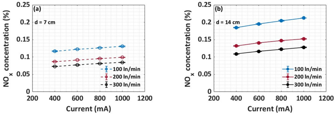
Figure 9. NO x concentration as a function of current, for three different flow rates and a distance between the electrodes of (a) 7 cm, and (b) 14 cm, in the large reactor in pin-to-pin configuration. Error bars are indicated but are too small to be visible.
