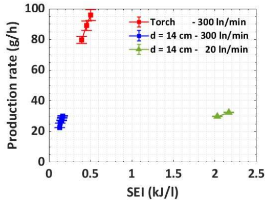
Figure 13. Total \text{NO}_x production rate as a function of SEI, for the three different reactors, i.e., small pin-to-pin, large pin-to-pin, and the large reactor in torch configuration. The conditions with the lowest EC are presented here.
