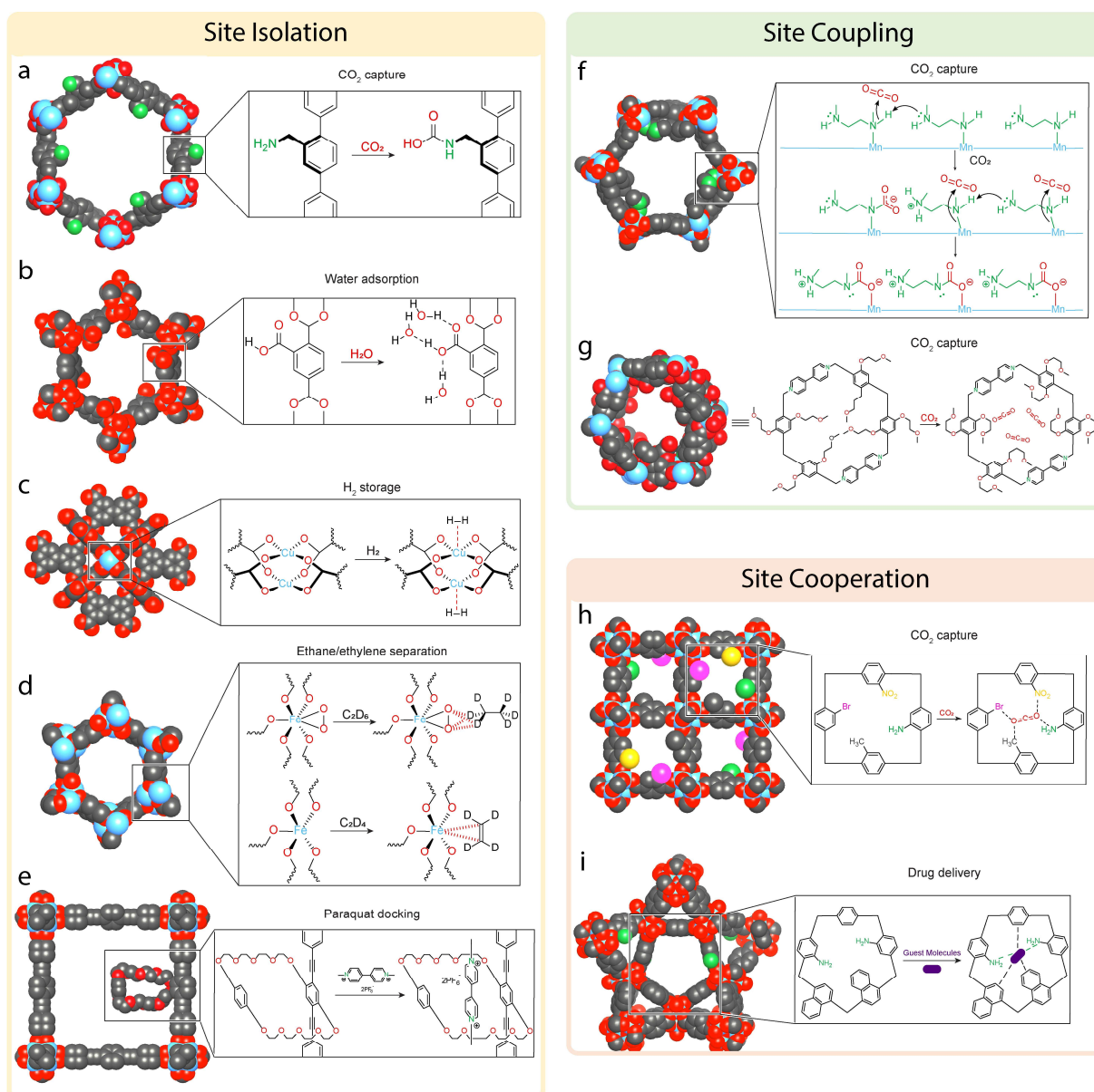
Figure 5. Site-specific functionalization of pores for guest binding. Through site isolation, functionalities work independently: the amine group for CO 2 capture (a); the carboxylate group for water adsorption (b); the open metal sites for H 2 storage (c) and ethane/ethylene separation (d); the macrocyclic crown ether for paraquat docking (e). Through site coupling, functionalities of the same type bind to guests in collaborative ways: diamine (f) and alkyl ethers (g) gate the adsorption of CO 2 . Through site cooperation, functionalities of different types bind to guests in collaborative ways: mixing methyl, amine, bromo, and nitro groups in one framework for CO 2 capture, outperforming the sum of every homogeneous component (h); mixing amine and benzene groups for tuning drug release rate (i). Color code: metal,
