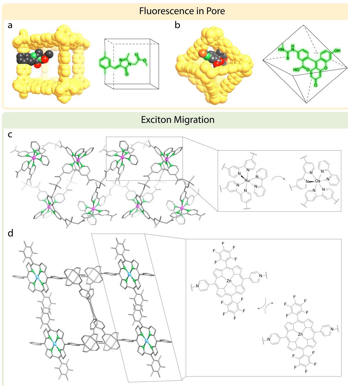
Figure 8. Pore functionalization for facilitating fluorescence and energy transfer. (a) A benzylidene imidazolidinone chromophore confined in a cubic pore. (b) Fluorescein confined in a octahedron pore containing a missing edge defect. (c) Triplet-triplet energy transfer between reticulated Ru and Os complexes through the Dexter mechanism. (d) Anisotropic alignment of the reticulated Zn-porphyrin for the Förster energy transfer. Color code: backbone encompassing chromophores, yellow; C, grey; O, red; N, green; S, orange; Ru/Os, magenta; Zn, blue. H atoms are omitted for clarity.
