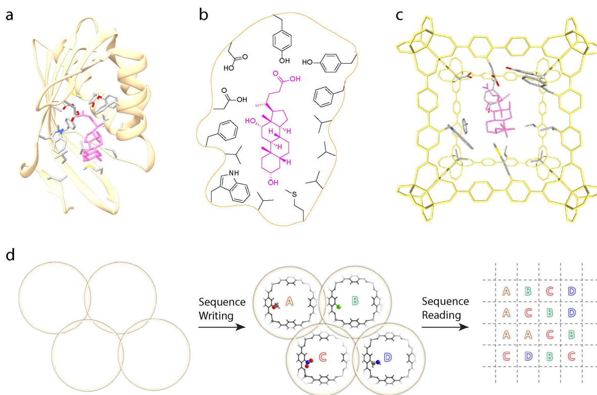
Figure 11. Approaching the structural complexity and sophistication of enzymes by functionalized frameworks. (a) The pocket of an enzyme ketosteroid isomerase complexed with a substrate deoxycholic acid (magenta). The polypeptide scaffold is depicted in yellow. Residues involved in substrate interaction are shown. (b) The chemical structure of the substrate and the relevant residues. (c) Functionalities are installed on the backbone of IRMOF-10 (yellow) for accommodating the binding of deoxycholic acid (magenta). Color code for the residues and functionalities: C, grey; O, red; N, blue; S, yellow. (d) Schematic illustration of functionality-sequence writing and reading by using synthetic tools and characterization techniques.
