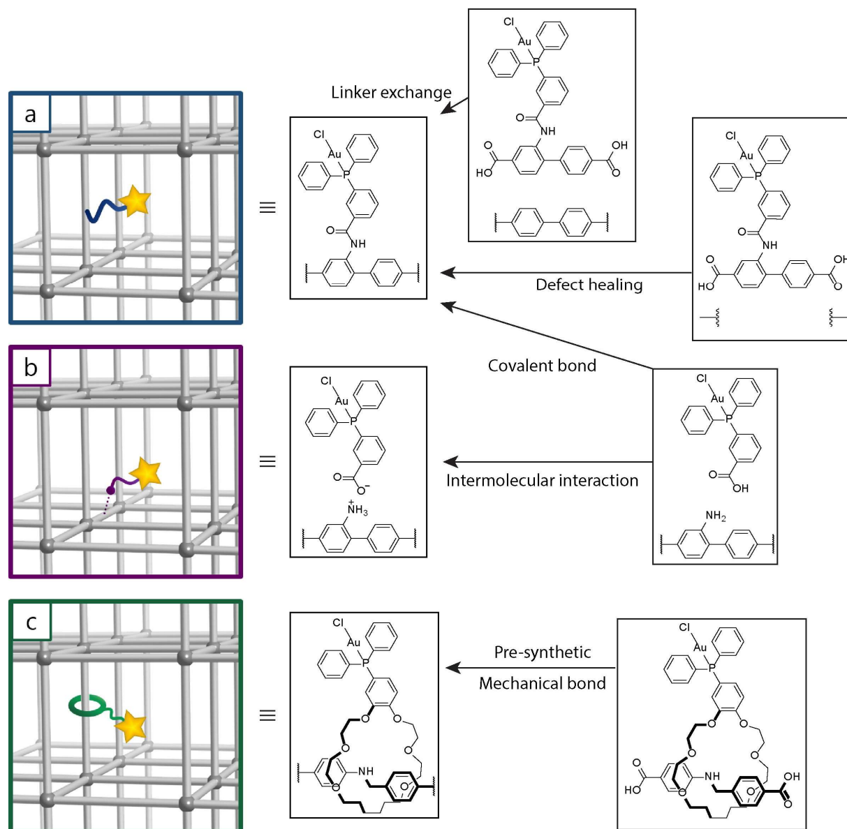
Figure 4. The chemistry of functionalizing a MOF in pcu net with chloro(triphenylphosphine)gold(I). (a) Covalent attachment can be achieved by grafting functionalites to the reactive moieties on the backbone though the formation of amide. Alternatively, linker molecules bearing the gold-phosphine complex can post-synthetically replace the native ones or occupy missing-linker defects. (b) Intermolecular interaction can be used for the adsorption of negatively charged gold-phosphine complex to the positively charged backbone. (c) Mechanical interlocking attaches the gold-phosphine complex to the
