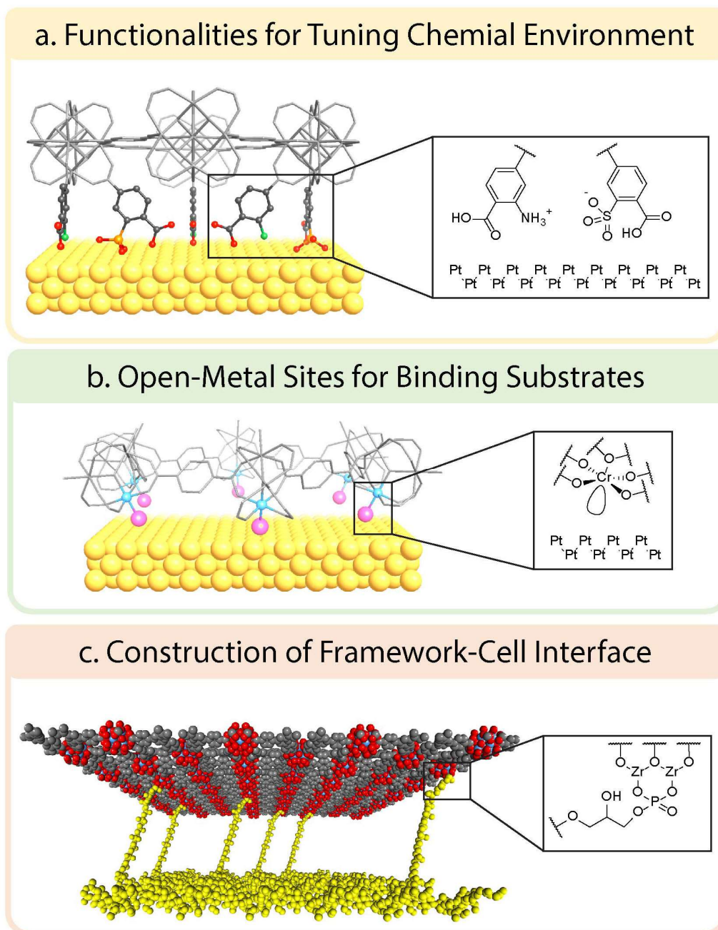
Figure 10. The functionalized, porous interface between frameworks and porous materials. (a) Organic functionalities appended on the framework backbone for tuning the environment of catalytic Pt surface. (b) Open metal sites for docking substrates in specific orientations with respect to catalytic Pt surface. (c) The polymeric phosphate units dangling from the bacterial cell wall coordinate to the unsaturated metal sites of Zr clusters on a MOF monolayer.
