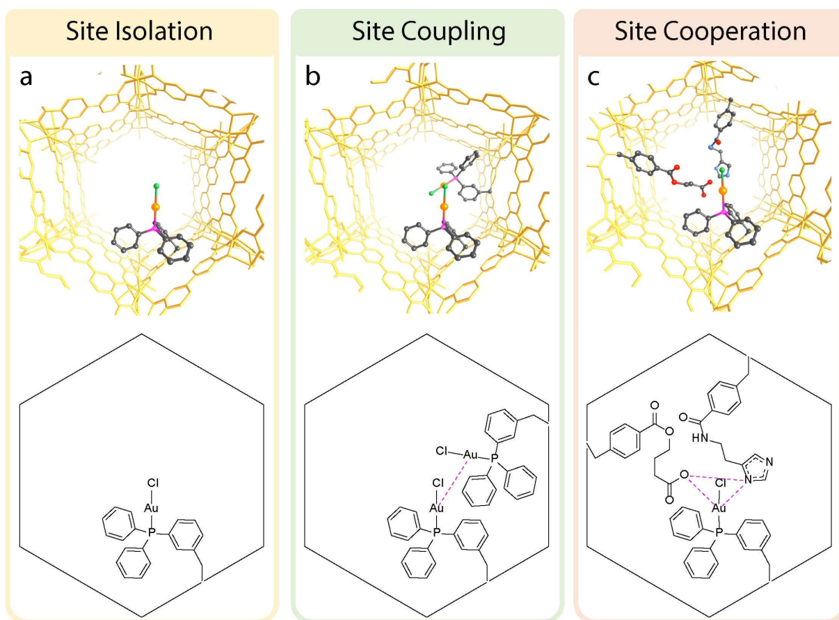
Figure 1. Pore functionalization strategies illustrated by the installation of chloro(triphenylphosphine)gold(I) in the hexagonal channel of IRMOF-74-II. The metal-phosphine complexes are appended onto the MOF backbone, being isolated (a), coupled (b), or cooperative with organic functionalities in close proximity (c). The backbone of IRMOF-74-II is presented in yellow sticks. The functionalities are illustrated in the ball-and-stick model. Color code: Au, orange; Cl, green; P, magenta; C, grey; O, red; N, blue. H atoms are omitted for clarity. The magenta dash lines in molecular structures indicate intermolecular interactions between functionalities.
