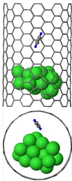
Figure 1. Ni 18 nanocluster and C 2 H 2 molecule inside (10,10) tube
