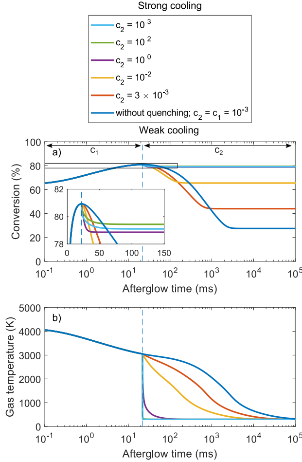
Figure 11: Time-evolution of the \text{CO}_2 conversion (a) and gas temperature (b), for different cooling rates, for a VT equilibrium plasma with SEI of 4 eV/molec. that is quenched at maximum \text{CO}_2 conversion. The plasma is initially subjected to weak cooling ( c_1 = 10^{-3} ), i.e. warm plasma. The cooling constants c_2 in the afterglow are indicated in the legend.
