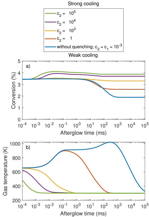
Figure 10: Time-evolution of the \text{CO}_2 conversion (a) and gas temperature (b), for different cooling rates in the afterglow, for a VT non-equilibrium plasma with SEI of 0.5 eV/molec. that is quenched at the plasma end. The plasma is initially subjected to weak cooling ( c_1 = 10^{-3} ), i.e. warm plasma. The cooling constants c_2 in the afterglow are indicated in the legend.
