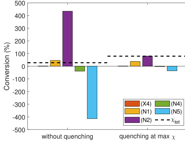
Figure 7: Total contribution of the dissociation and recombination reactions to the conversion for an equilibrium plasma with SEI of 4 eV/molec. that is quenched at maximum conversion (right), and that was subjected to weak cooling ( c = 10^{-3} ). The case without quenching (left) is shown as a reference. The horizontal dashed lines indicate the final \text{CO}_2 conversion. In contrast to the non-equilibrium plasma of fig. 6, electron impact dissociation (X4) has a negligible contribution to the final \text{CO}_2 conversion.
