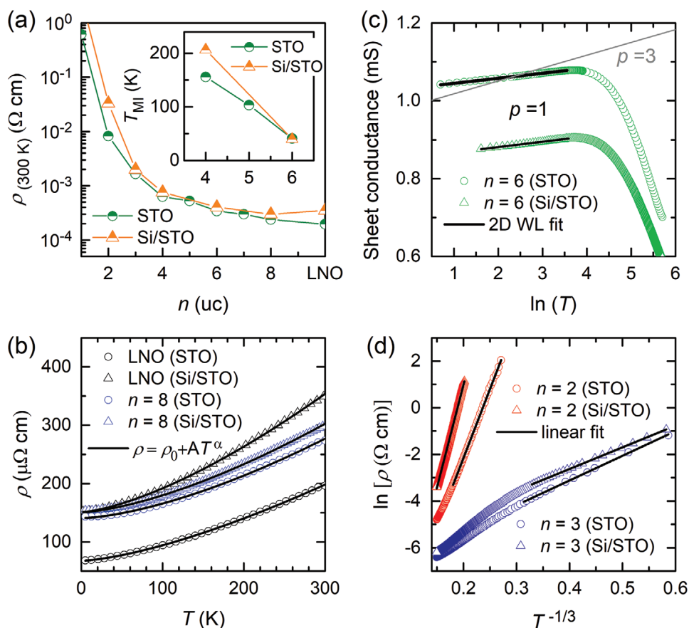
Figure 4. Modeling conduction mechanisms in LNO/LFO SLs. a) Room-temperature resistivity \rho_{(300\text{ K})} and T_{\text{MI}} (inset) as a function of n . b) \rho - T curves of the metallic LNO single films and n=8 SLs grown on STO and Si/STO. The solid lines are fits to \rho = \rho_0 + AT^\alpha . c) Sheet conductance plotted against \ln(T) for the n=6 SLs, with fittings to the 2D WL model. The sheet conductance is calculated for the LNO individual layer considering a parallel resistor model. The fittings give \rho \approx 1 for both samples, and the case of \rho \approx 3 is shown by the gray line. d) Logarithm of resistivity as a function of T^{-1/3} for the SLs with n=2 and 3, with fittings to the 2D VRH model.
