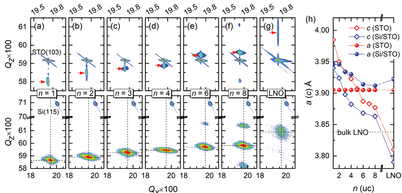
Figure 2. Strain contrast between LNO/LFO SLs grown on STO and Si/STO. a–g) RSMs of (103)_{pc} reflection for SLs grown on STO (top panels) and Si/STO (bottom panels). The black dotted lines in the bottom panels mark Q_x and Q_z positions of the SLs on Si/STO. h) Extracted a and c as a function of n .
