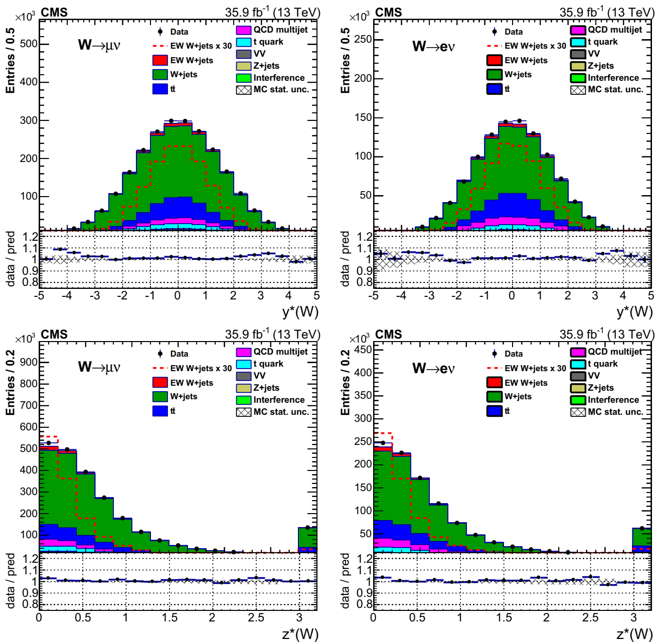
Fig. 6 Distributions of the “Zeppenfeld” variables y^*(W) (upper) and z^*(W) (lower) after event preselection in the muon (left) and electron (right) channels. In all plots the first and last bins contain overflow events
