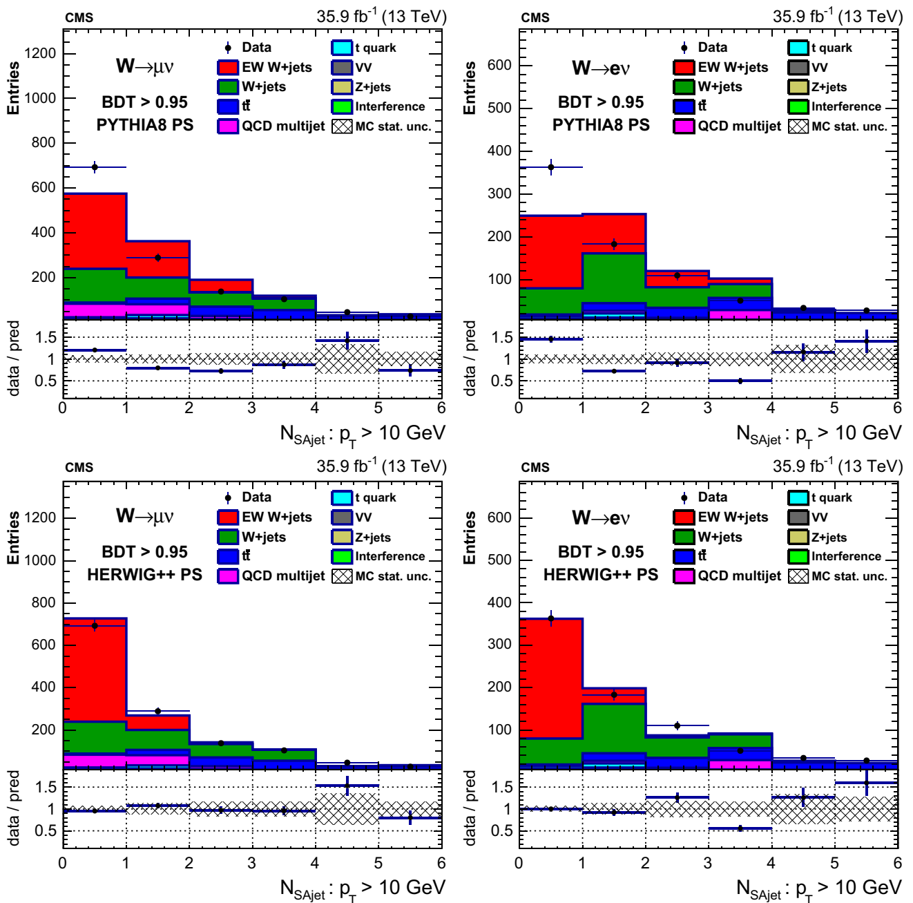
Fig. 20 Number of soft activity jets with p_T > 10 GeV in the rapidity gap for BDT > 0.95 in the muon (left) and electron (right) channels including signal with PYTHIA parton showering (upper) and HERWIG++ parton showering (lower). In all plots the last bin contains overflow events
