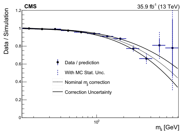
Fig. 3 Data divided by simulation as a function of \ln(m_{jj}/\text{GeV}) in a signal-depleted control sample with R(p_T) > 0.2 . This distribution is fit by a third-order polynomial (solid black line) in order to derive a correction on the simulation m_{jj} prediction. The points are varied by the uncertainty, including the effect of the limited number of simulated events and refitted in order to derive the systematic variations on the correction (dashed lines) corresponding to a standard deviation (SD)
