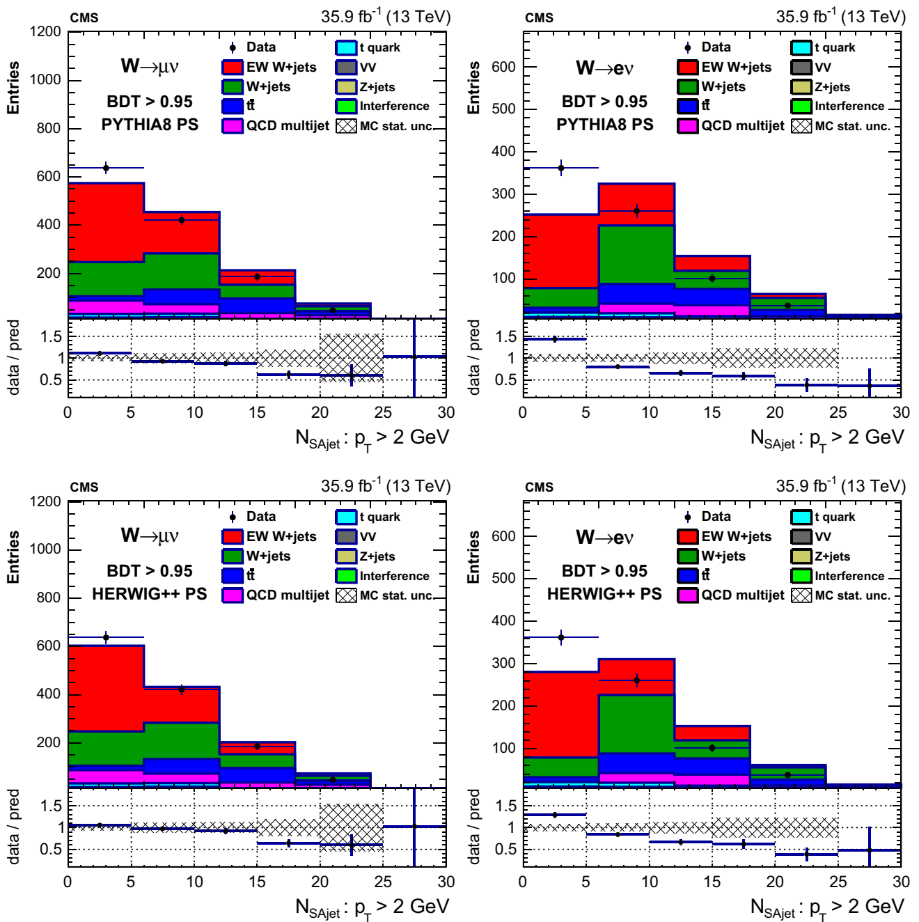
Fig. 22 Number of soft activity jets with p_T > 2 \text{ GeV} in the rapidity gap for \text{BDT} > 0.95 in the muon (left) and electron (right) channels including signal with PYTHIA parton showering (upper) and HERWIG++ parton showering (lower)
