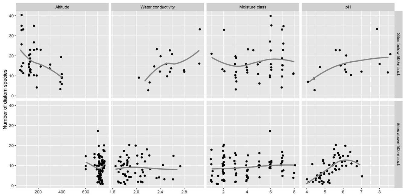
Figure 5 —A scatterplot showing the relation between species richness and environmental variables (elevation, pH, moisture, and conductivity), with the samples divided into two groups, according to elevation (0–500 m a.s.l. and above 500 m a.s.l.). Note that the species richness is clearly increasing with increasing pH and conductivity in the samples of the lower elevations.
