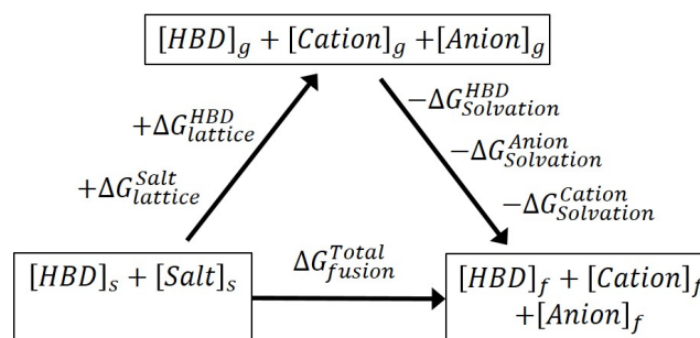
Figure 6: Born-Fajans-Haber cycle of NADES melting, lattice and solvation energies.
