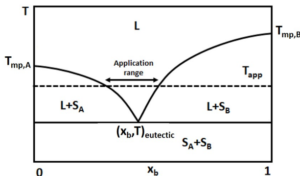
Figure 4: T-x phase diagram of simple eutectic behavior: the diagram shows the change of the system's melting point ( T ) as the function of molar ratio of constituent B ( x_B ) in the mixture. T_{mp,A} , T_{mp,B} are the melting points of the pure A and B constituents, T_{app} is the temperature of the given application, L is the liquid phase, while S_A and S_B are the solid phases of constituent A and B. (x_{B,T})_{eutectic} indicates the eutectic composition and temperature of the mixture.
